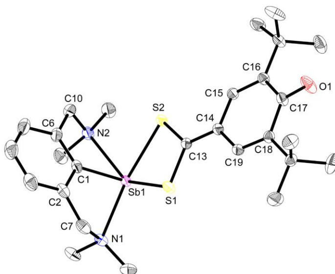
Figure 6. Representation of the molecular structure of [\{NCN^{Me^d}\}Sb(S_2C-C_6H_2-{}^tBu_2-3,5-O-4)] ( 13 ). H atoms and non-interacting pyridine molecules omitted for clarity. Ellipsoids at the 50% probability level. Selected distances (Å) and angles (°): Sb1–C1 = 2.1429(17), Sb1–N1 = 2.5492(15), Sb1–N2 = 2.6003(15), Sb1–S1 = 2.5505(5), Sb1–S2 = 2.5723(5), C17–O1 = 1.248(2), S1–C13 = 1.7369(17), S2–C13 = 1.7364(17), C13–C14 = 1.395(2), C14–C15 = 1.429(2), C14–C19 = 1.431(2), C15–C16 = 1.358(2), C16–C17 = 1.474(2), C17–C18 = 1.475(2), C18–C19 = 1.355(2); C1–Sb1–N1 = 72.36(6), C1–Sb1–N2 = 71.69(6), C1–Sb1–S1 = 96.31(5), C1–Sb1–S2 = 96.96(5), N1–Sb1–N2 = 126.95(5), N1–Sb1–S1 = 78.32(4), N1–Sb1–S2 = 144.59(4), S1–Sb1–N2 = 143.01(4), S1–Sb1–S2 = 69.240(15), S2–Sb1–N2 = 77.48(3).
