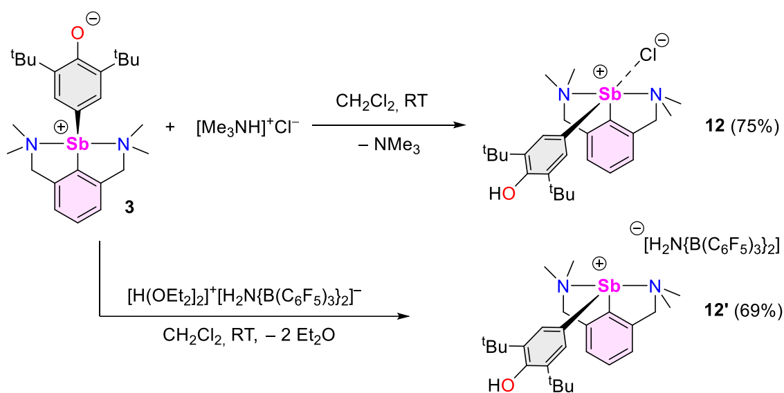
Scheme 4. Synthesis of [ \{NCN^{Me4}\}Sb(C_6H_2-{}^1Bu_2-3,5-OH-4)[X] ] (X = Cl, 12 ; H_2N\{B(C_6F_5)_3\}_2 , 12' ).
