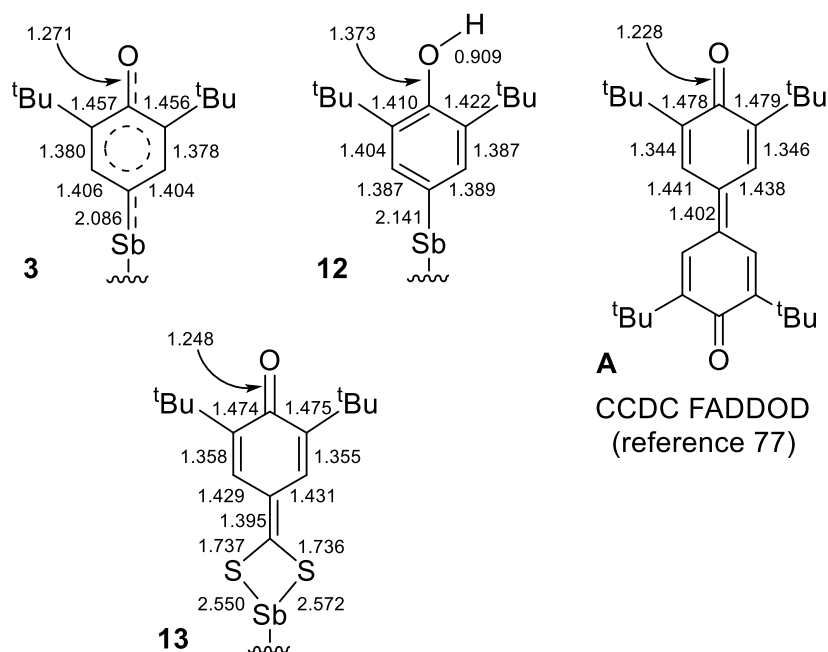
Figure 7. Selected interatomic distances in 3 , 12 , 13 and A . Supporting ligand framework {NCN Me4 } - and ESD's omitted for clarity.
