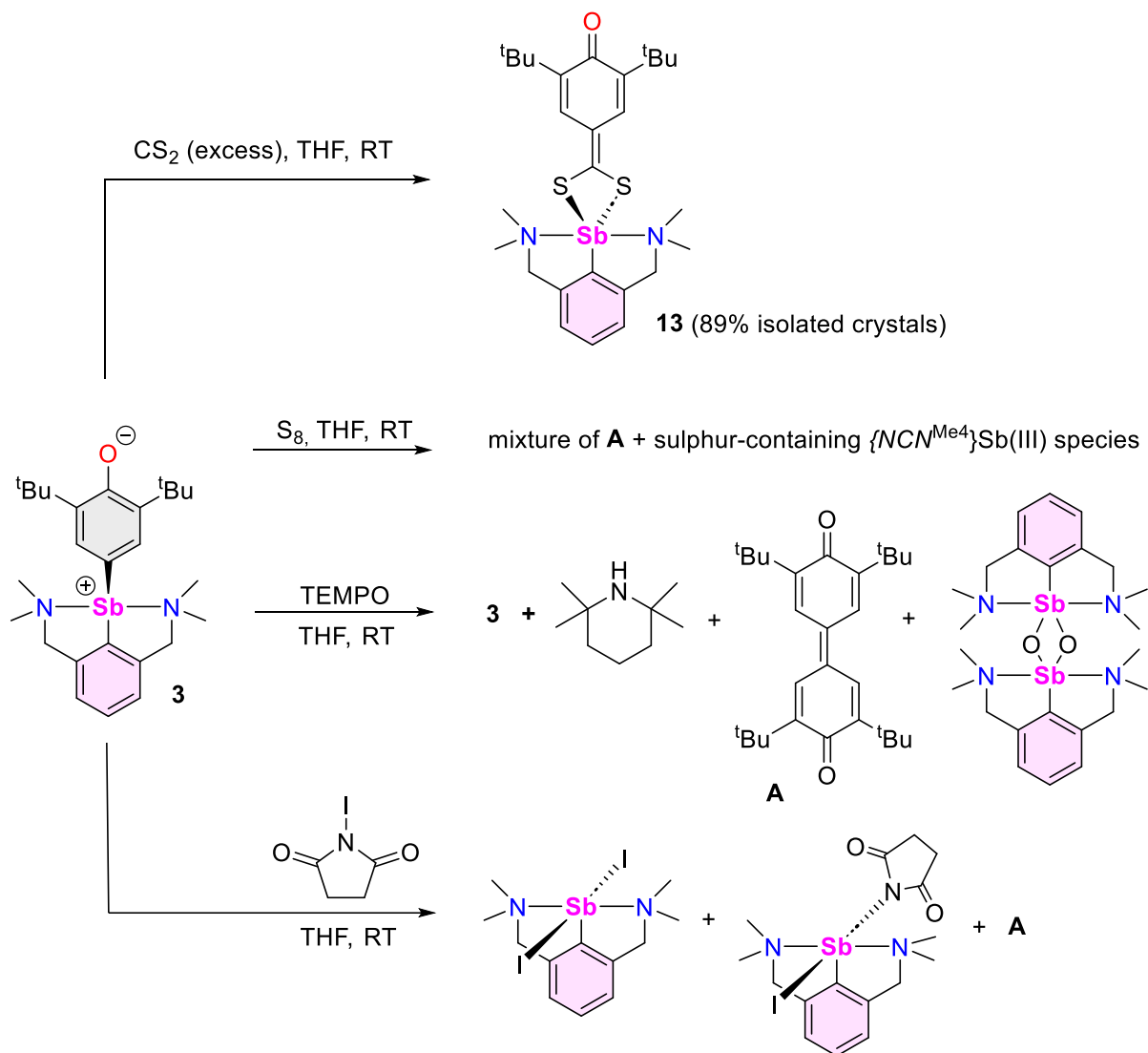
Scheme 7. Probing the reactivity of 3 .
