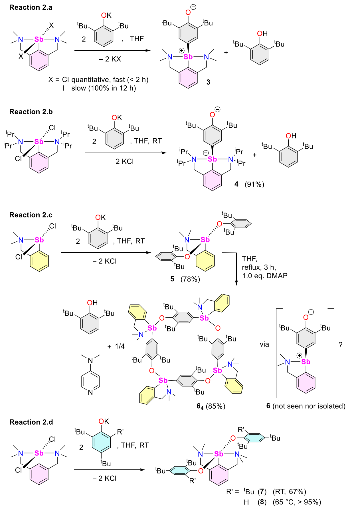
Scheme 2. Reactions of Sb(III) dihalides with potassium phenolates.
