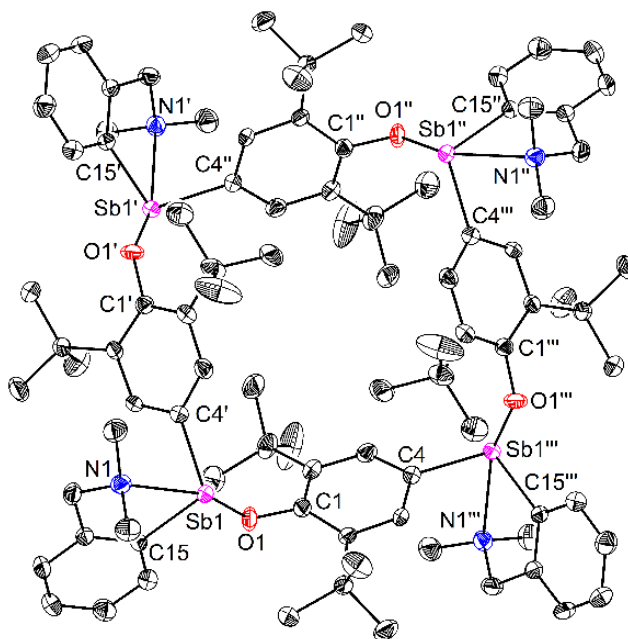
Figure 4. Representation of the molecular structure of [\{CN^{Me2}\}Sb(C_6H_2\text{-}^t\text{Bu}_2\text{-3,5-O-4})_4] ( 6a ). H atoms omitted for clarity. Ellipsoids at the 50% probability level. Selected distances (Å) and angles (°): Sb1–C4' = 2.121(5), Sb1–C15 = 2.157(4), Sb1–N1 = 2.574(4), Sb1–O1 = 2.088(4), C1–O1 = 1.346(5); C4'–Sb1–O1 = 99.36(16), C4'–Sb1–C15 = 98.36(16), C4'–Sb1–N1 = 82.47(15), C15–Sb1–N1 = 72.87(15), C15–Sb1–O1 = 84.46(15), N1–Sb1–O1 = 157.25(12).
