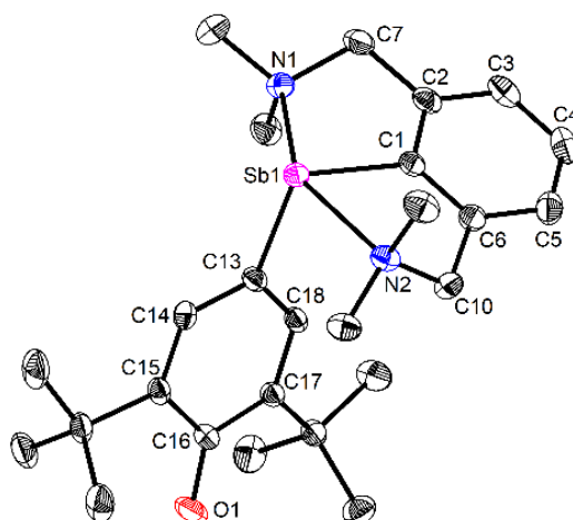
Figure 3. View of the molecular structure of [\{\text{NCN}^{\text{Me}4}\}\text{Sb}(\text{C}_6\text{H}_2\text{-}^t\text{Bu}_2\text{-}3,5\text{-O-}4)] ( 3 ). H atoms omitted for clarity. Ellipsoids at the 50% probability level. Only one of the two enantiomers ( pR_{\text{N1}} , pR_{\text{N2}} ) 49 in the asymmetric unit is shown. Selected distances (Å) and angles (°): \text{Sb1-C1} = 2.1134(13) , \text{Sb1-C13} = 2.0862(12) , \text{Sb1-N1} = 2.4458(11) , \text{Sb1-N2} = 2.4436(11) , \text{C13-C14} = 1.4063(17) , \text{C13-C18} = 1.4047(17) , \text{C14-C15} = 1.3803(17) , \text{C15-C16} = 1.4572(18) , \text{C16-C17} = 1.4559(17) , \text{C17-C18} = 1.3777(17) , \text{C16-O1} = 1.2708(16) ; \text{C1-Sb1-C13} = 101.02(5) , \text{C1-Sb1-N1} = 73.94(4) , \text{C1-Sb1-N2} = 74.16(4) , \text{C13-Sb1-N1} = 96.54(4) , \text{C13-Sb1-N2} = 89.09(4) , \text{N1-Sb1-N2} = 148.10(4) .
