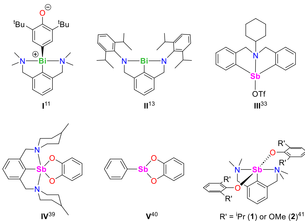
Figure 1. Selected examples of known Sb(III) and Bi(III) relevant to the present work.
