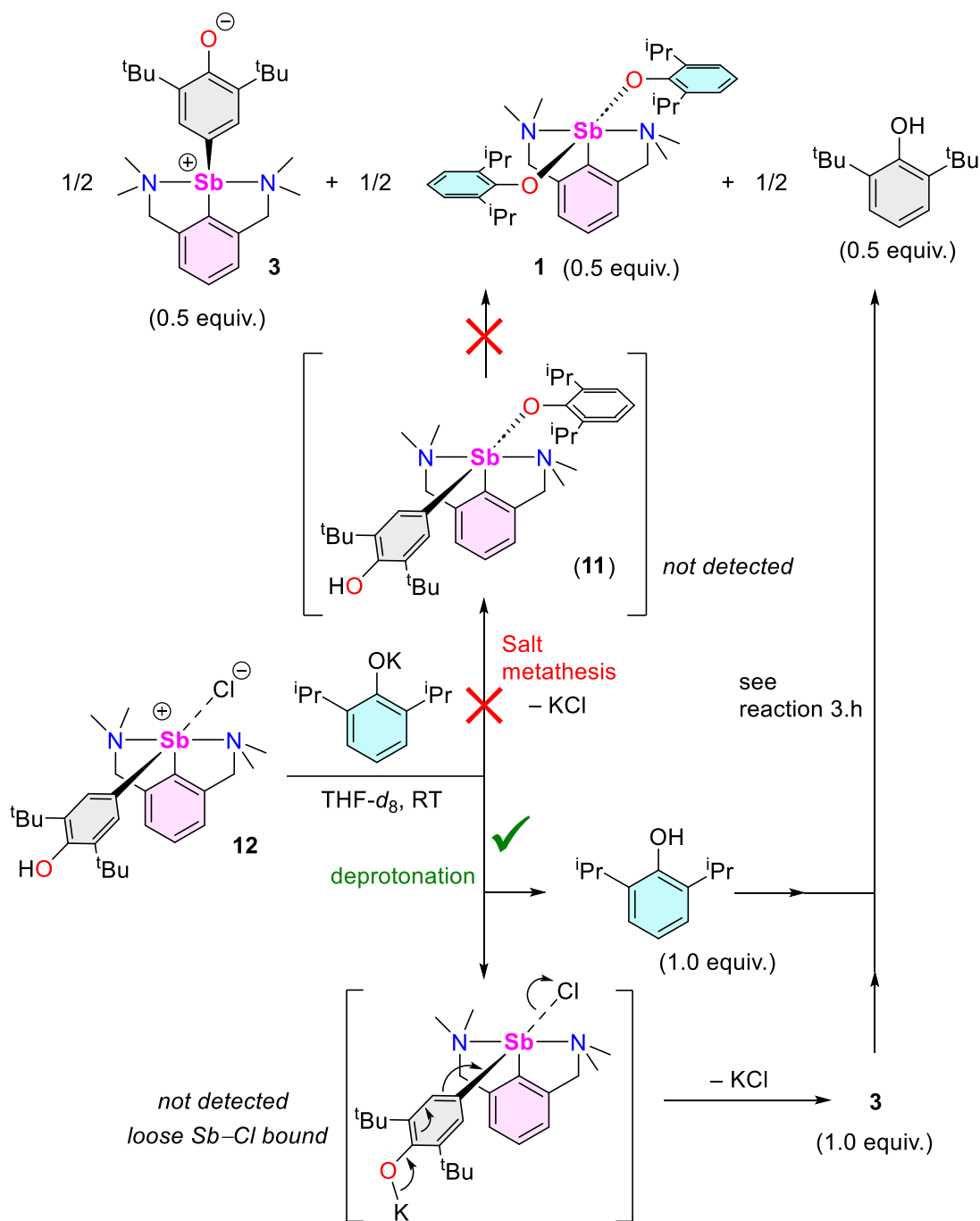
Scheme 5. Reaction of [\{NCN^{Me^4}\}\text{Sb}(\text{C}_6\text{H}_2\text{-}^t\text{Bu}_2\text{-}3,5\text{-OH-}4)(\text{Cl})] ( 12 ) with [\{2,6\text{-}^i\text{Pr}_2\text{-C}_6\text{H}_3\text{O}\}\text{K}] , highlighting the two potential mechanistic pathways.
