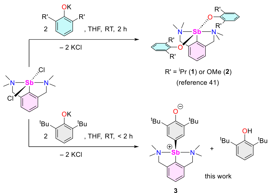
Scheme 1. Synthesis of [\{NCN^{Me4}\}Sb(C_6H_2-tBu_2-3,5-O-4)] ( 3 ).
