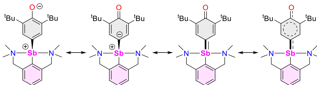
Figure 2. Mesomeric forms of [\{NCN^{Me4}\}Sb(C_6H_2-tBu_2-3,5-O-4)] ( 3 ).
