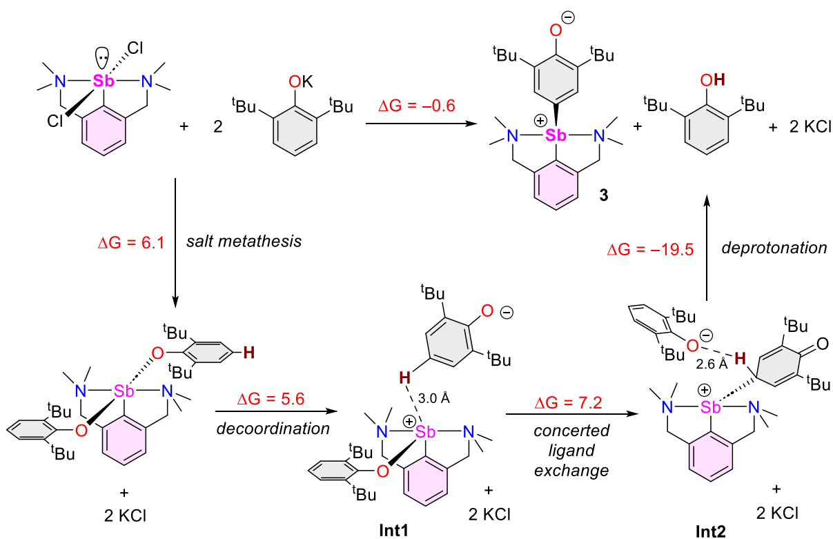
Scheme 6. Proposed pathway for the formation of 3 based on both experimental and computational data. The free energies at 298 K are given in kcal mol -1 . They were calculated assuming solvent (THF) effects (see Computational Details).
