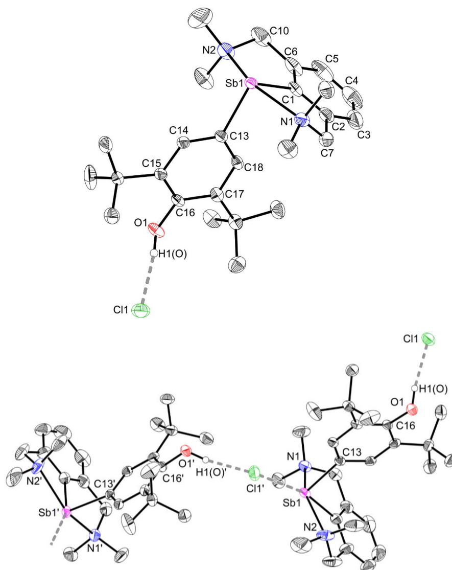
Figure 5. Top: representation of the molecular structure of [\{NCN^{Me4}\}Sb(C_6H_2-{}^tBu_2-3,5-OH-4)]Cl ( 12 ). Bottom: arrangement of two adjacent units in the lattice. H atoms (except that on O atoms) and non-interacting CH_2Cl_2 molecules omitted for clarity. Ellipsoids at the 50% probability level. Selected distances (Å) and angles (°): Sb1–C1 = 2.106(4), Sb1–C13 = 2.141(4), Sb1–N1 = 2.398(4), Sb1–N2 = 2.453(4), Sb1–Cl1' = 3.6761(14), C13–C14 = 1.387(5), C13–C18 = 1.389(5), C14–C15 = 1.404(5), C15–C16 = 1.410(5), C16–C17 = 1.422(5), C17–C18 = 1.387(5), O1–C16 = 1.373(4), O1–H1(O) = 0.909(6), Cl1–H1(O) = 2.154(34); C1–Sb1–C13 = 95.52(15), C1–Sb1–N1 = 74.59(15), C1–Sb1–N2 = 74.41(18), C13–Sb1–N1 = 90.80(13), C13–Sb1–N2 = 90.55(14), N1–Sb1–N2 = 148.95(14).
