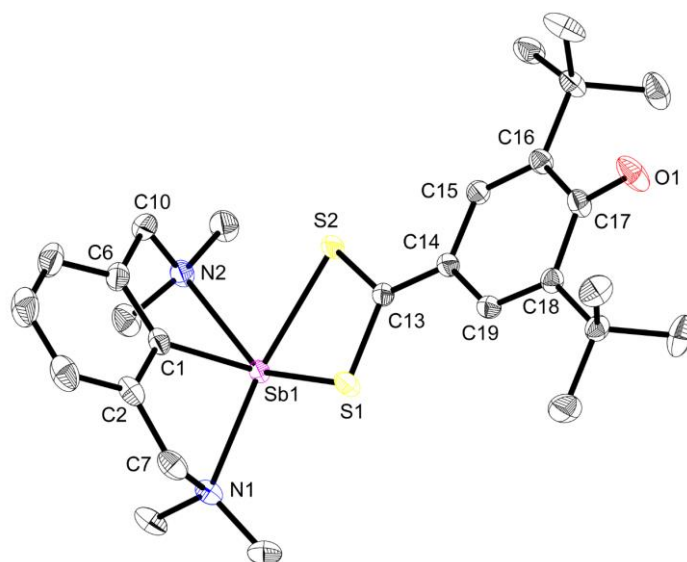
Figure 6. Representation of the molecular structure of [\{NCN^{Me^d}\}Sb(S_2C-C_6H_2-tBu_2-3,5-O-4)] ( 13 ). H atoms and non-interacting pyridine molecules omitted for clarity. Ellipsoids at the 50% probability level. Selected distances (Å) and angles (°): Sb1–C1 = 2.1429(17), Sb1–N1 = 2.5492(15), Sb1–N2 = 2.6003(15), Sb1–S1 = 2.5505(5), Sb1–S2 = 2.5723(5), C17–O1 = 1.248(2), S1–C13 = 1.7369(17), S2–C13 = 1.7364(17), C13–C14 = 1.395(2), C14–C15 = 1.429(2), C14–C19 = 1.431(2), C15–C16 = 1.358(2), C16–C17 = 1.474(2), C17–C18 = 1.475(2), C18–C19 = 1.355(2); C1–Sb1–N1 = 72.36(6), C1–Sb1–N2 = 71.69(6), C1–Sb1–S1 = 96.31(5), C1–Sb1–S2 = 96.96(5), N1–Sb1–N2 = 126.95(5), N1–Sb1–S1 = 78.32(4), N1–Sb1–S2 = 144.59(4), S1–Sb1–N2 = 143.01(4), S1–Sb1–S2 = 69.240(15), S2–Sb1–N2 = 77.48(3).
