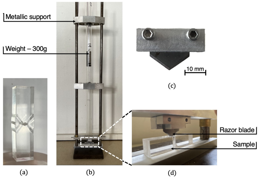
Figure 8: PMMA DCDC sample preparation (a) Trial to create pre-cracks by cyclic compressive loading, the material shows significant plastic strain before crack initiation at the poles of the hole (b) Setup designed for tapping a triangular razor blade (c) positioned on the sample as shown in (d).
