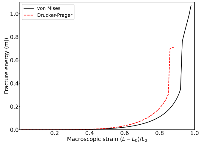
Figure B.25: Pre-cracked SENB test: Comparison of the energy dissipated by fracture as the crack progresses for a material defined by a von Mises or Drucker-Prager plasticity criterion.
