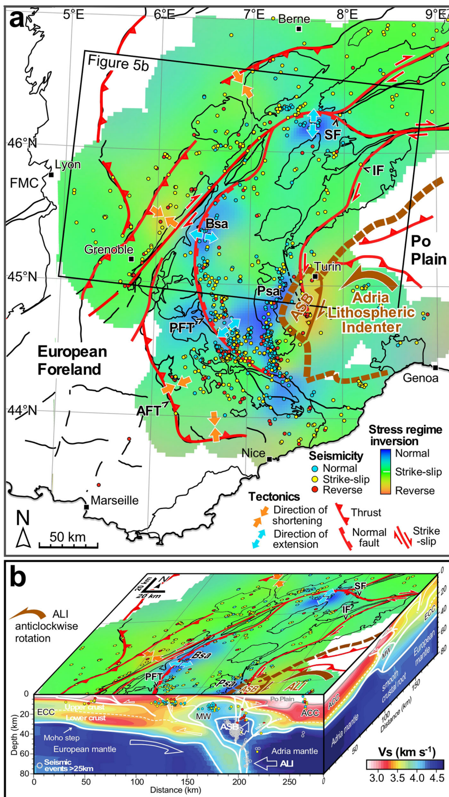
Fig. 5 Seismotectonic and structural model of the W-Alps. a Seismotectonic map of the W-Alps showing the main tectonic structures accommodating the indentation of Adria plate associated with the global Adria - Europe convergence. The overall strike-slip deformation regime is controlled by the Adria anticlockwise rotation. Stress redistribution on the European crust is variably accommodated due to its internal anisotropy related to Variscan inheritance. b Interpretative 3D block diagram showing the relationships between surface strain partitioning and crustal scale geometry revealed by Vs tomography. The main seismic arcs are named Bsa and Psa for the Briançonnais and for the Piemontais seismic arc respectively. The other acronyms are the same as in Fig. 1b.
