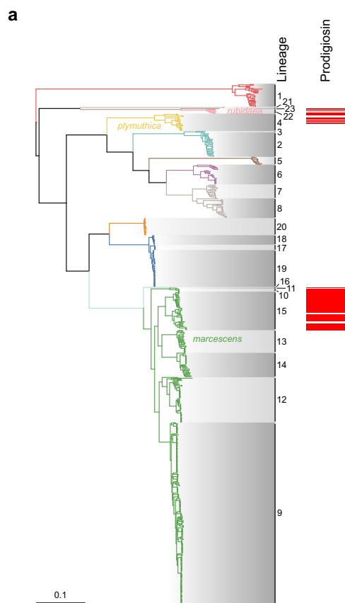
Fig. 7 | The prodigiosin gene cluster is present variably across Serratia and in different genomic loci. a Prodigiosin ( pig ) gene clusters identified using Ham-burger are plotted against the maximum-likelihood phylogeny of Serratia shown in
