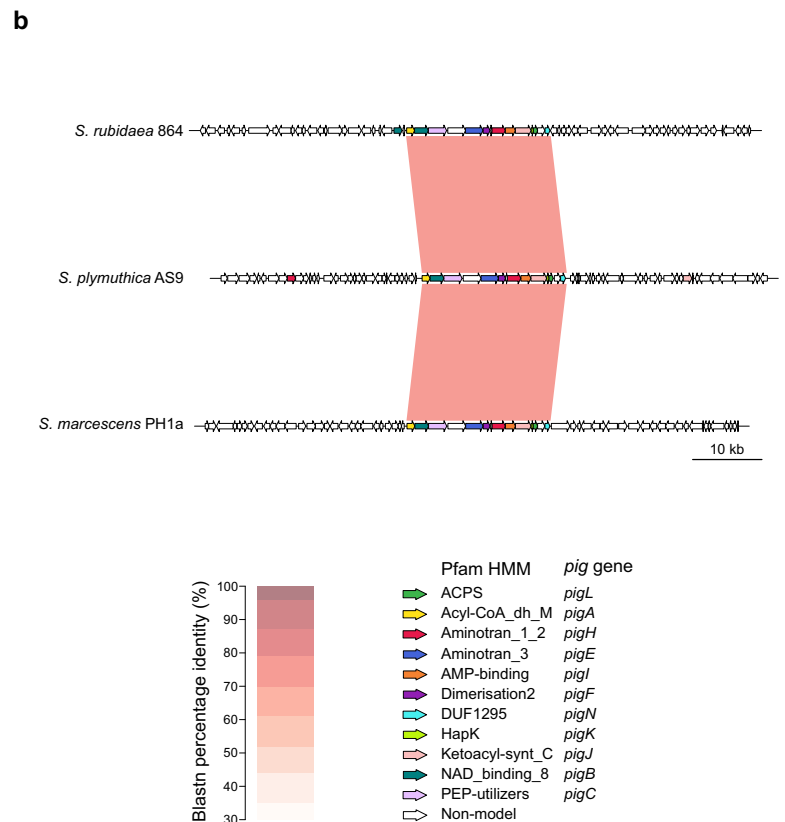
Fig. 1. b Pairwise blastn comparison of pig loci (core pig cluster +/-20 kb) from representative members of the three species containing pig genes, extracted using Ham-burger.
