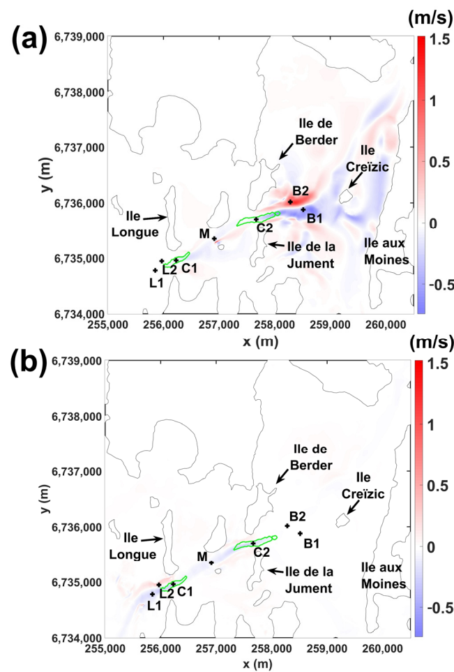
Figure 6. Perturbation of the current velocity magnitude in m/s (scenario No. 1) at peak flood (a) and ebb (b) during a spring tide (8 April 2020). Locations of tidal farms are indicated with green lines. Coordinates are in meters (EPSG 4326).
