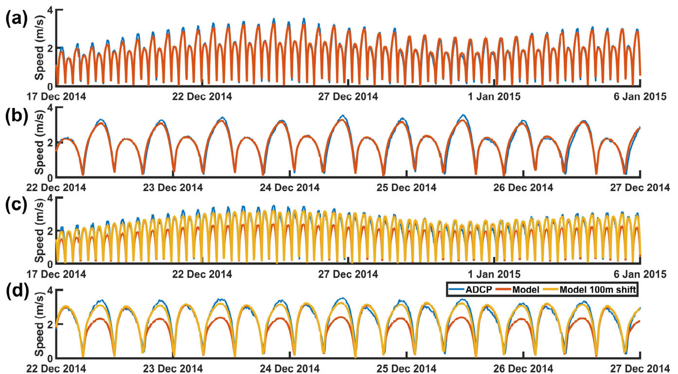
Figure 3. Comparison between depth-averaged current speeds predicted by the model (red and yellow curves) and measured by ADCPs (blue curves). Subplots (a,b) correspond to the site located south of “Ile Longue” (same location but different time series lengths). Subplots (c,d) correspond to the site located south of “Berder” (same location but different time series lengths). The yellow curves were obtained by moving the point where the data were extracted by 100 m.
