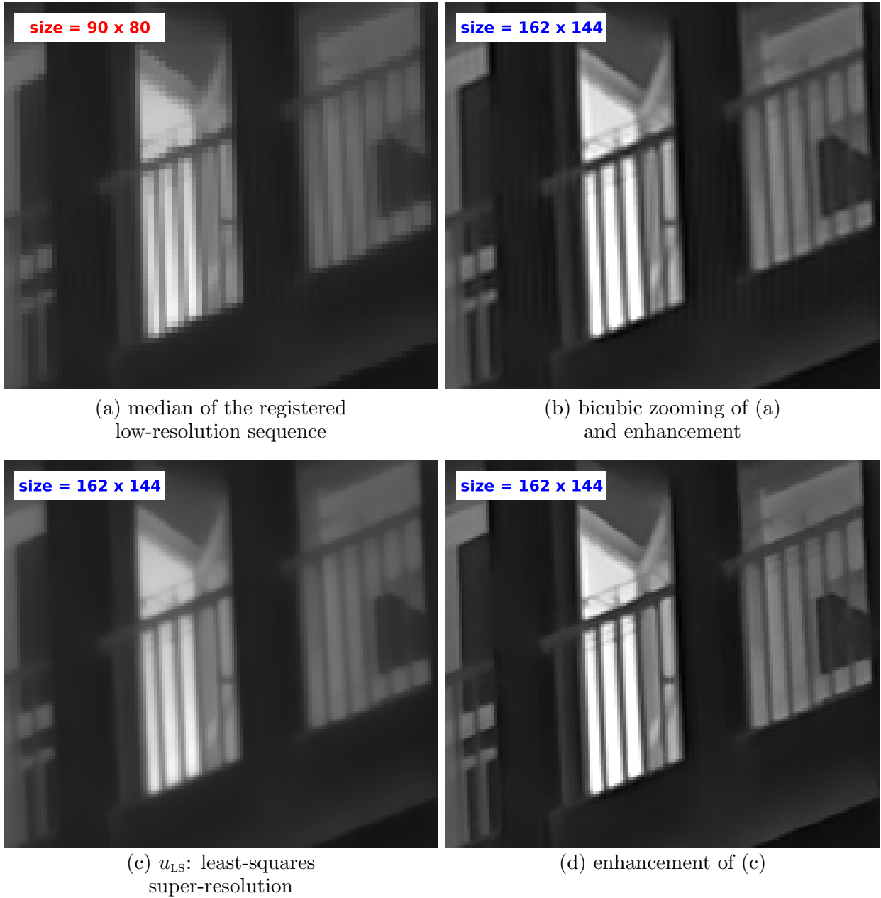
Figure 17: Effect of the enhancement filter \psi_5 on the super-resolved image. We consider again the thermal infrared sequence u_0 of L = 500 low-resolution images with size 200 \times 200 (see Section 5.5 and Figure 12). We display in (a) a 90 \times 80 close-up of the shift-and-median reconstruction (that is, the pointwise median of the registered sequence of low-resolution images). By magnifying this reconstruction with a factor 1.8 in both directions (bicubic zooming) we get an image with size 360 \times 360 on which we apply the enhancement filter defined by \psi_5 , leading to the close-up image (b). We can see that the enhancement yields an image with better contrast and a better level of details, but at the same time, amplified artifacts. We display in (c) and (d) equivalent close-ups for the least-squares super-resolution image u_{\text{LS}} obtained from u_0 (zoom factors: z_x = z_y = 1.8 ). It is interesting to see that the enhancement of u_{\text{LS}} , in addition to its ability to better reveal super-resolution details, does not produce any noticeable artifact.
