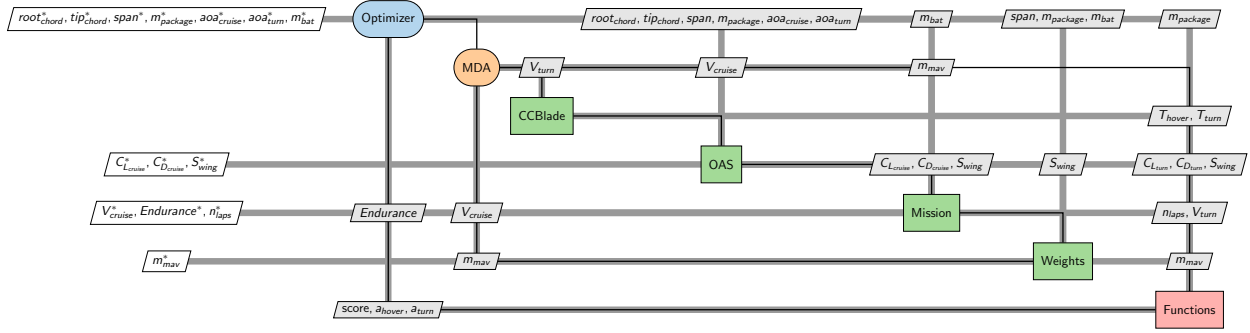
Fig. 21: Extended design structure matrix of the refined tail-sitter process.
