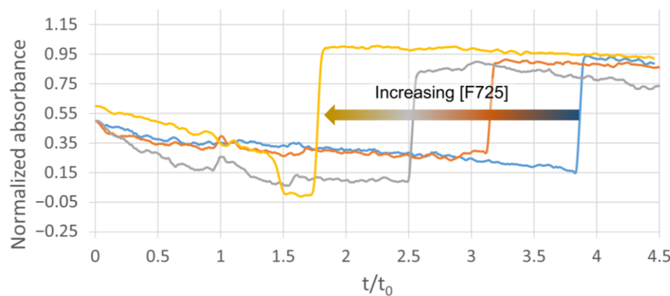
Figure 6. Frontal affinity chromatograms of caffeine (25 \mu\text{M} ) on affinity column (+A2A) in absence (blue plot) and in presence of increasing concentrations of competitor (F725): 200 \mu\text{M} (orange plot), 500 \mu\text{M} (grey plot), and 2 mM (yellow plot). Experiment carried out in 20 mM mobile-phase ammonium acetate with pH of 7.4. UV detection occurred at 260 nm.
