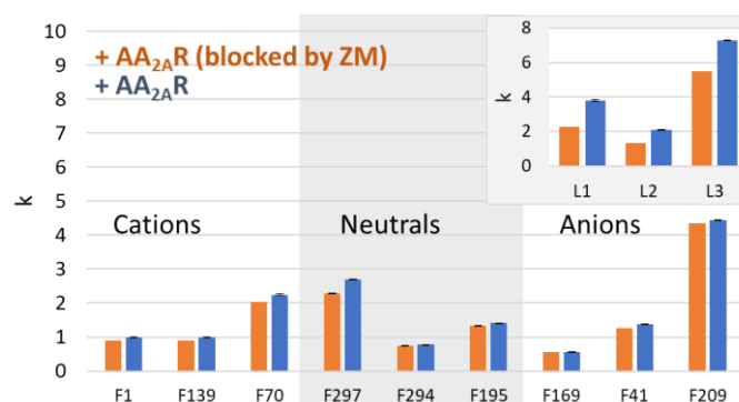
Figure 5. Bar charts comparing the retention factors of the 12 test fragments measured on columns functionalized with NDs (POPC) with the (+AA 2A R) receptor and on the same column after saturation of the membrane protein by ZM241385. The experiments were carried out in 20 mM mobile-phase ammonium acetate with a pH of 7.4.
