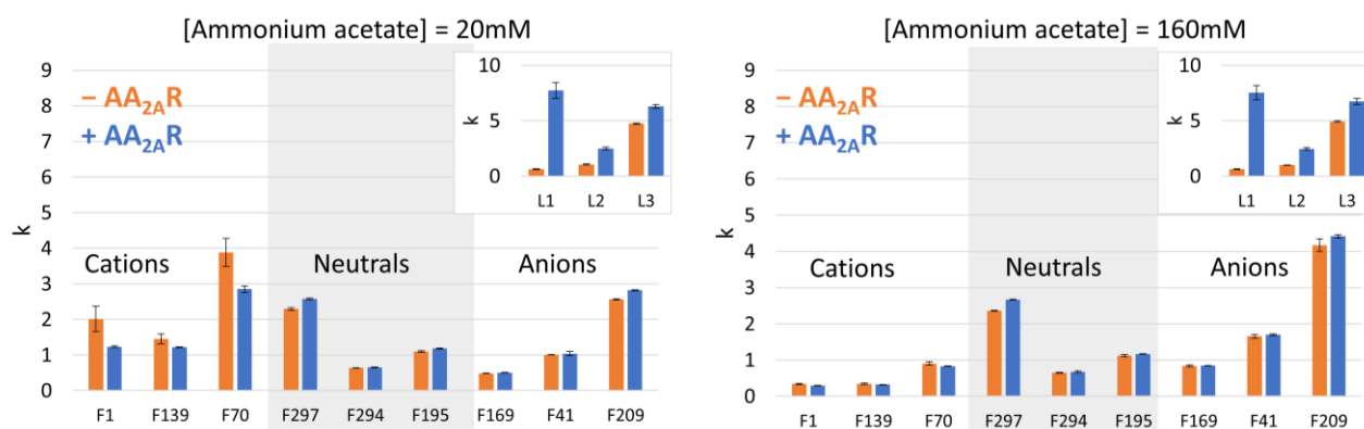
Figure 4. Bar charts comparing the retention factors measured on columns functionalized with POPC/POPG NDs with (+) and without (–) AA 2A R for ligand (insert, L1, L2, and L3) and non-ligand fragments. Experiments were performed either in 20 mM mobile-phase ammonium acetate with a pH of 7.4 ( left ) or in 160 mM mobile-phase ammonium acetate with a pH of 7.4 ( right ).
