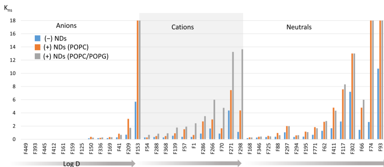
Figure 2. Plot of the non-specific retention factor k_{ns} of the 39 fragments on poly(GMA-co-MBA) monoliths in the absence (-) and presence (+) of NDs, measured in 20 mM mobile-phase ammonium acetate (pH of 7.4). The fragments were classified by their charge state and ordered by increasing logD values (pH of 7.4).
