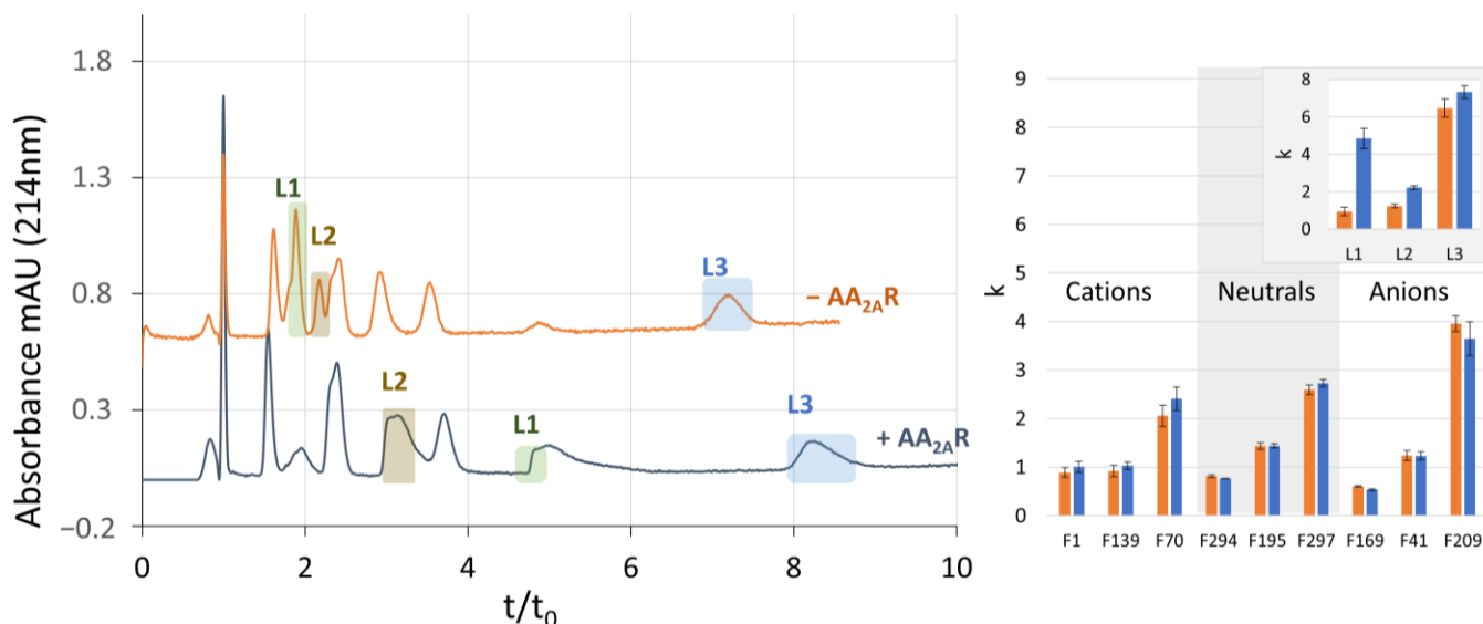
Figure 3. Evaluation of empty NDs (POPC) as control columns. (Left): Chromatograms of the set of 12 fragments (9 non-ligands and 3 ligands) injected on the empty-ND (POPC)-functionalized column (-AA 2A R) and the affinity-ND (POPC) column (+AA 2A R). Column length, 8.5 cm; mobile phase, 20 mM ammonium acetate (pH of 7.4); fragment concentration, 50 \mu M. (Right): Graphs showing the variation in the retention factors on the empty (orange) and affinity (blue) columns for the 9 non-ligands and the 3 known ligands of AA 2A R (insert, L1, L2, and L3). Error bars are the standard deviation calculated from three repetitions.
