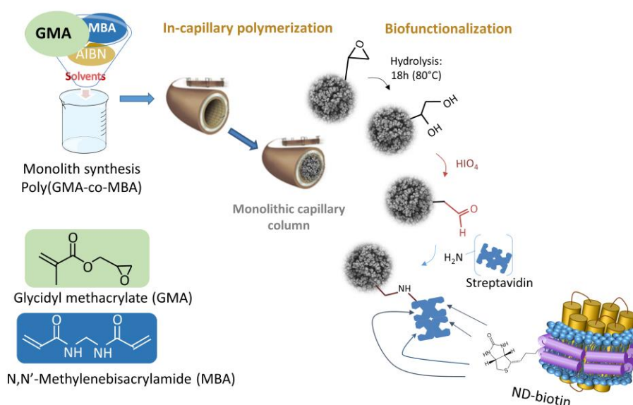
Figure 1. Schematic representation of the in-capillary poly(GMA-co-MBA) synthesis, surface functionalization, and immobilization of biotinylated nanodiscs.
