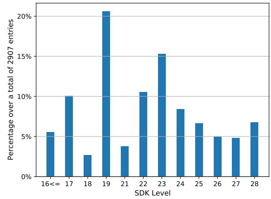
Fig. 1. SDK Distribution
