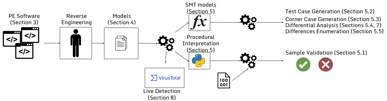
Figure 1: An overview of our analysis process.
