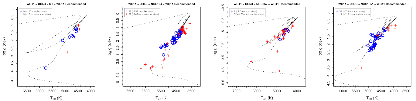
Fig. 4. T_{\text{eff}} - \log g diagrams for the globular clusters M2, NGC 104, NGC 362, and NGC 1851.
