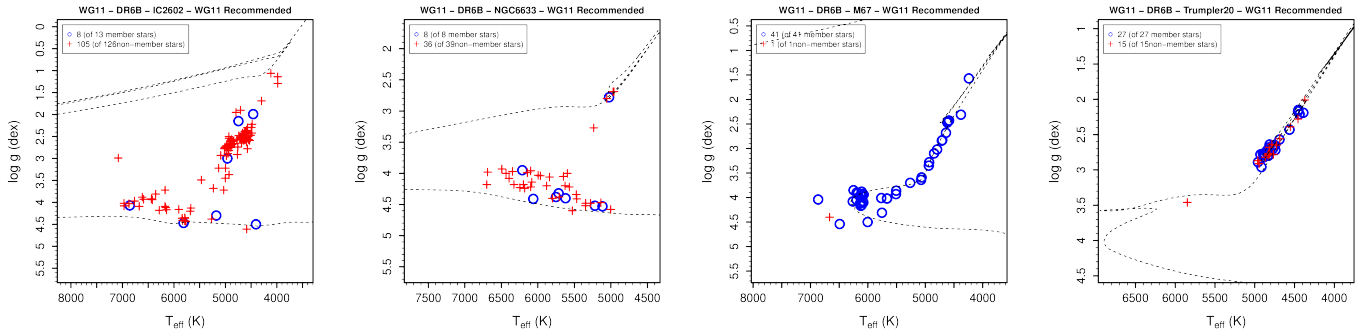
Fig. 3. T_{\text{eff}} - \log g diagrams for the open clusters IC 2602, NGC 6663, M67, and Trumpler 20.
