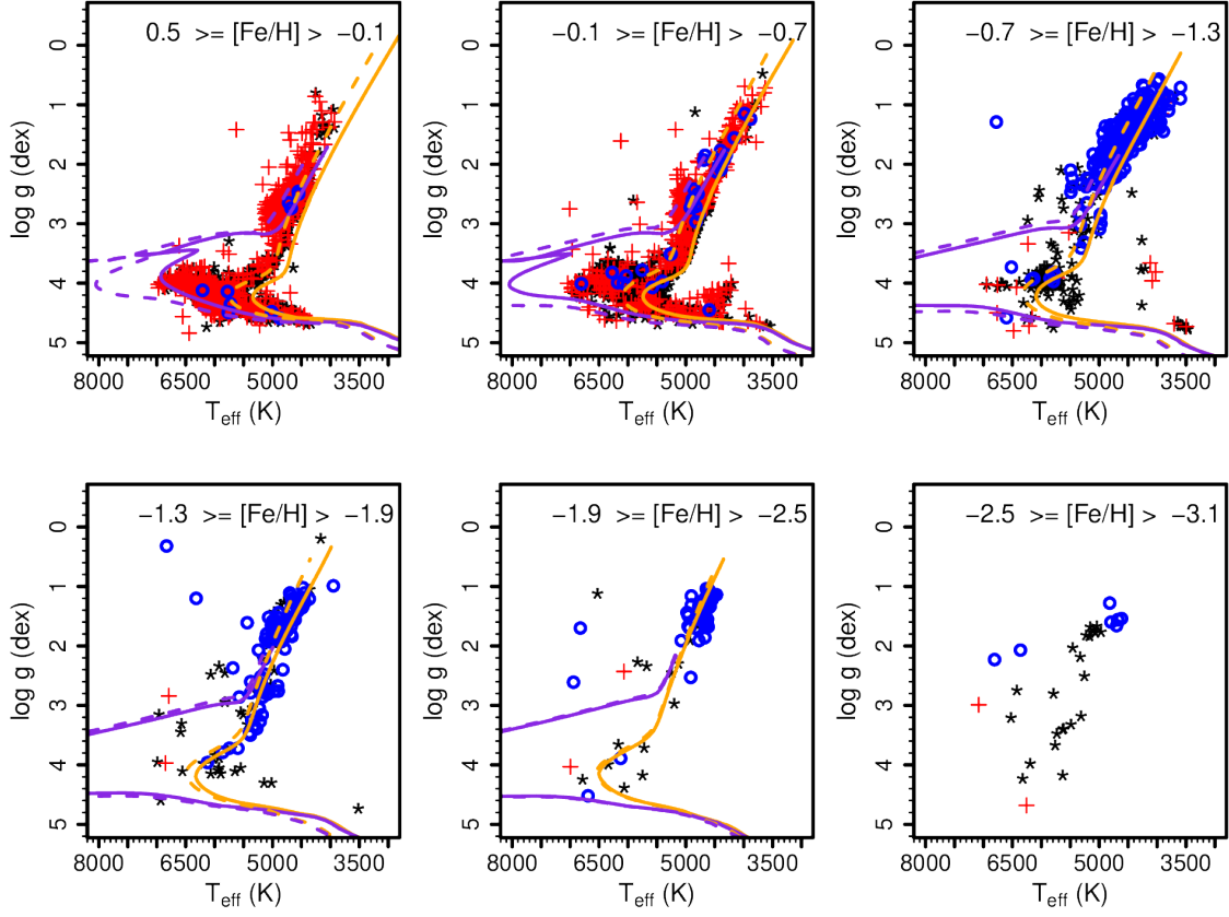
Fig. 2. T_{\text{eff}} - \log g diagram with the WG11 recommended results. PARSEC isochrones (Bressan et al. 2012) are shown for ages of 1 and 12.5 Gyr (violet and orange, respectively) and for the minimum and maximum metallicity indicated in each panel (dashed and solid lines, respectively). Red crosses are stars in open clusters, blue circles are stars in globular clusters, and the black starred symbols are the remaining stars.
