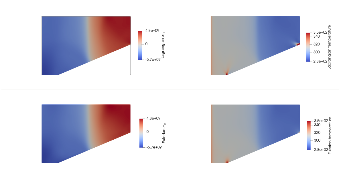
Figure 14: Maps of the stress component \sigma_{11} and the temperature in the wedge computational domain, extracted from both the Lagrangian and Eulerian numerical solutions at time t \approx 1.1 \times 10^{-4} seconds.
