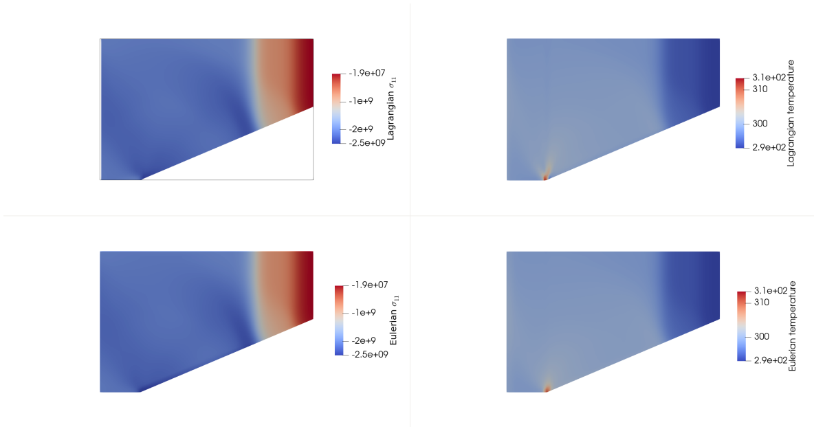
Figure 13: Maps of the stress component \sigma_{11} and the temperature in the wedge computational domain, extracted from both the Lagrangian and Eulerian numerical solutions at time t \approx 3.8 \times 10^{-5} seconds.
