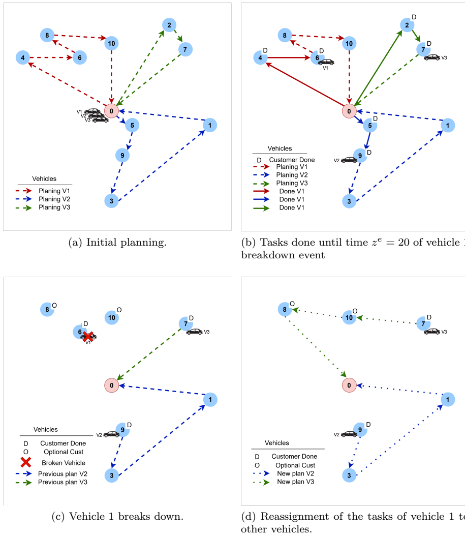
Figure 2: Example of the execution of the dynamic approach when vehicle 1 breaks down in the middle of its route.
