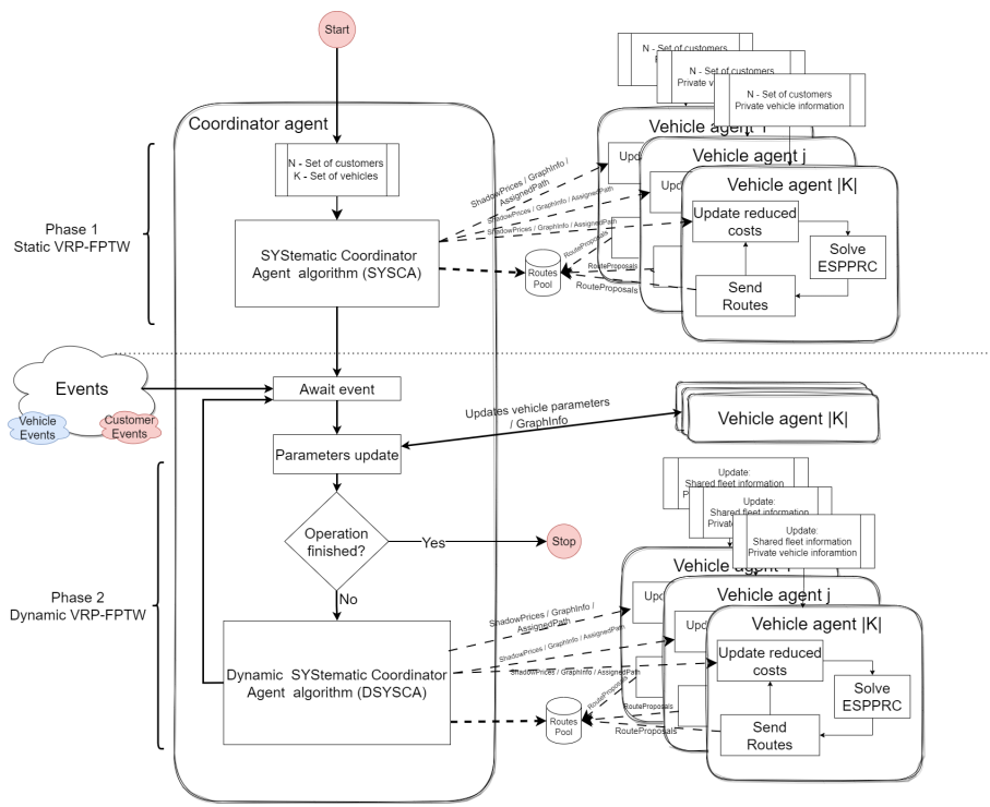
Figure 1: DIMASA architecture for the Static/Dynamic VRP-FPTW.
