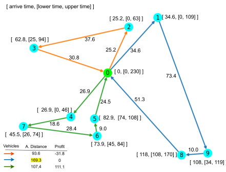
Figure 3: Example of generation of the parameters for the VRP-FPTW with 9 consumer vertices and 3 vehicles.
