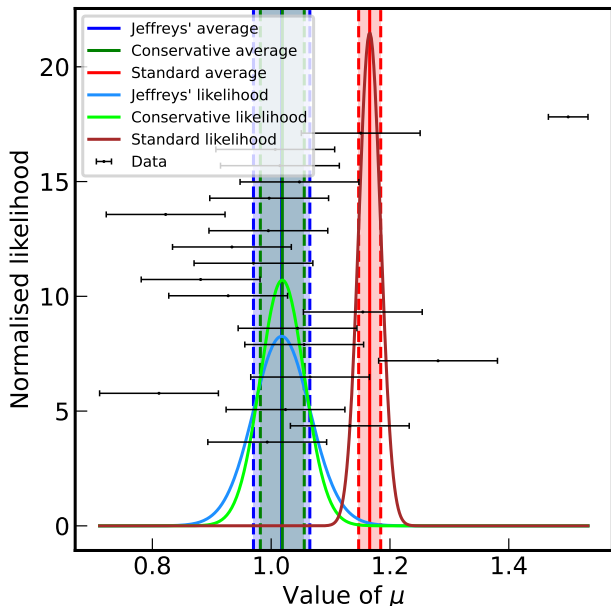
FIG. 2. Final likelihood distribution for the data set 3 together with the input values.
