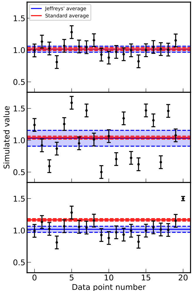
FIG. 1. Standard and Jeffreys' weighted averages of different simulated data sets: data randomly sampled from a normal distribution (top), and with the addition of a random bias (middle) or an outlier (bottom).
