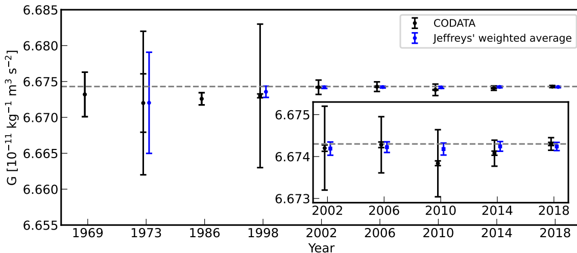
FIG. 3. Comparison between the official CODATA values [18–26] of the Newtonian constant and the values obtained by the Bayesian weighted average using Jeffreys’ prior. CODATA values obtained from single measurements are presented alone, as no weighted average could be performed. The small error bar of the CODATA values indicates the uncertainty calculated by the standard weighted average, and the large one indicates the recommended uncertainty. The horizontal dashed line corresponds to the latest CODATA value (2022 edition [27], equal to the 2018 edition one).
