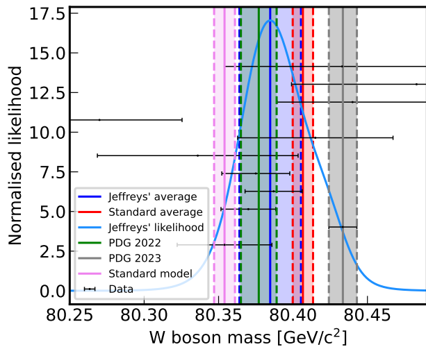
FIG. 8. Final likelihood distribution (in linear scale) corresponding to the PDG measurement selection for the W boson mass. The PDG official values of the 2022 and 2023 edition are also reported together with the Standard Model prediction. As can be seen, our Jeffreys’ weighted average agrees within 1.5 standard deviations with the predicted value.
