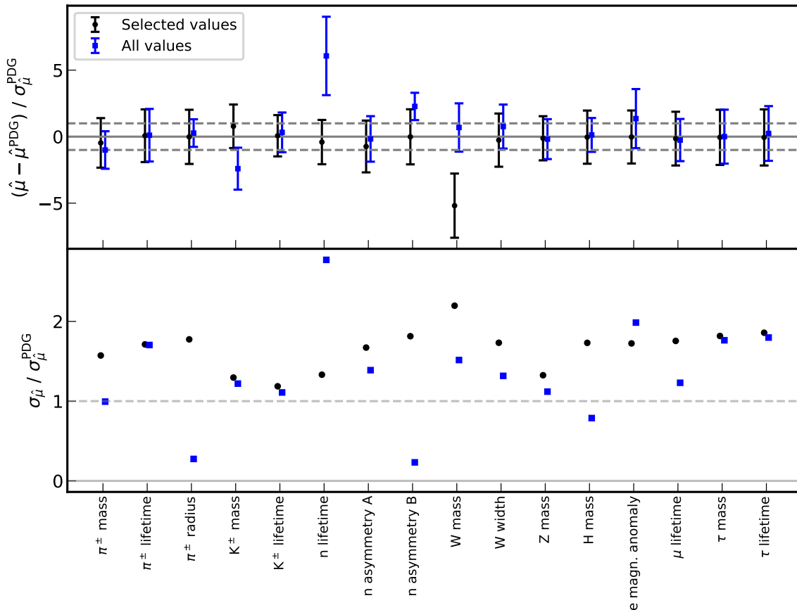
FIG. 5. Top: Comparison between the values obtained by the Bayesian weighted average using Jeffreys' prior and the official PDG values of several particle properties [30, 31]. All values are normalised to the PDG uncertainties. The two dashed horizontal lines correspond to \hat{\mu} - \hat{\mu}^{\text{PDG}} = \pm \sigma_{\hat{\mu}}^{\text{PDG}} , i.e. to \pm 1 in the relative scale. Bottom: Ratio between the uncertainties obtained for the Jeffreys' weighted average and the official PDG uncertainties
