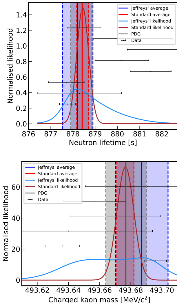
FIG. 6. Final likelihood distribution (in linear scale) corresponding to the PDG measurement selection for the neutron lifetime (top) and the charged kaon mass (bottom). In these cases, the final probability distribution generated by the Bayesian method is highly asymmetric and cannot be approximated by a Gaussian distribution. For these cases, the whole probability distribution should be considered for further inference analyses instead of any kind of weighted averages.
