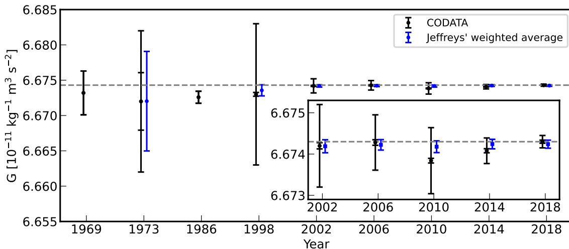
FIG. 3. Comparison between the official CODATA values [18–26] of the Newtonian constant and the values obtained by the Bayesian weighted average using Jeffreys’ prior. CODATA values obtained from single measurements are presented alone, as no weighted average could be performed. The small error bar of the CODATA values indicates the uncertainty calculated by the standard weighted average, and the large one indicates the recommended uncertainty. The horizontal dashed line corresponds to the latest CODATA value (2022 edition [27], equal to the 2018 edition one).
