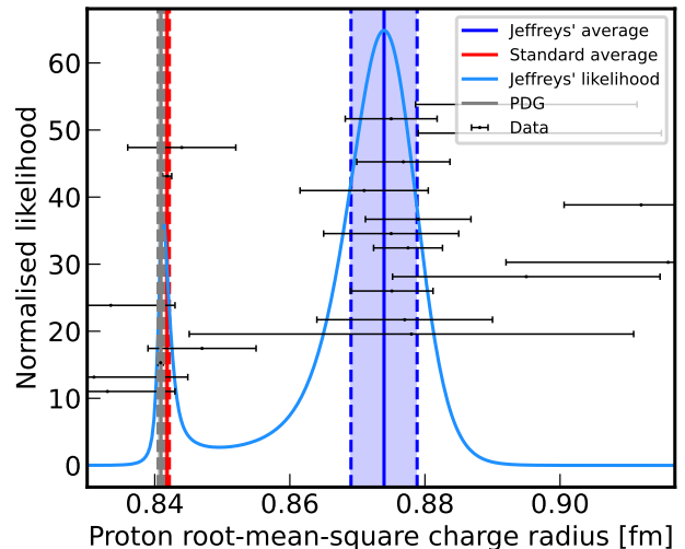
FIG. 7. Final likelihood distribution (in linear scale) corresponding to the PDG measurement selection for the proton radius. The PDG official value is also reported, which is very close to the standard weighted average. Due to the bimodality of the final probability distribution, using a weighted average is completely inappropriate.
