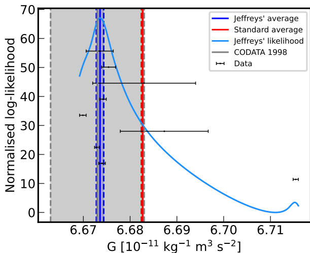
FIG. 4. Final likelihood distribution (in log-scale) of the measurements of the Newtonian constant included in the CODATA 1998 compilation [21]. The CODATA 1998 recommended value is also reported (in gray), which differs from the standard weighted average for the considered measurements (in red).
