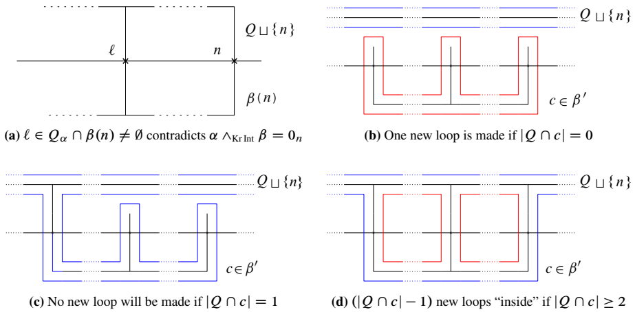
Figure 6. Panels (b), (c), and (d) describe (6) with |c| = 3 . The upper black lines represent Q \sqcup \{n\} and the lower black lines c . Preexisting loops of meandric systems are represented by blue lines, and new loops produced by adding c are indicated by red lines.
