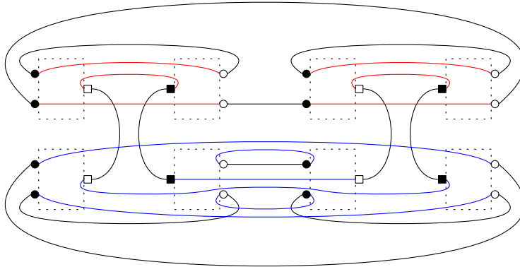
Figure 9. The diagram \mathcal{D}_{\alpha=(1)(2),\beta=(12)} as a term in the graphical Wick expansion of \mathbb{E} \text{Tr} Z^2 . This diagram consists of 6 d -dimensional loops (3 corresponding to the top (red) pictures and 3 corresponding to the bottom (blue) ones) and of 1 \ell -dimensional loop.
