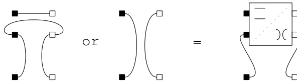
Figure 13. The LHS shows the Choi–Jamiołkowski matrices of the two possible operations: X \mapsto \text{Tr}[X]I_\ell or X \mapsto X , respectively.
