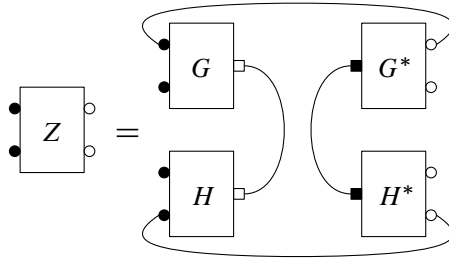
Figure 8. A graphical representation of the bi-partite matrix Z = [\Phi_G \otimes \Phi_H](\omega_\ell) . Round labels represent the space \mathbb{C}^d , while square labels represent \mathbb{C}^\ell .
