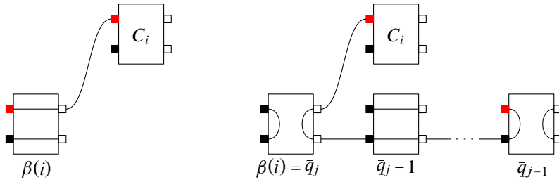
Figure 12. Following the top outputs (in red) of the C -boxes in the diagram \text{Tr}_{\beta,\gamma}[C_1^{\mathcal{Q}}, C_2^{\mathcal{Q}}, \dots, C_{n-1}^{\mathcal{Q}}, C_n] . Left: \beta(i) \notin \bar{\mathcal{Q}} ; right: \beta(i) = \bar{q}_j \in \bar{\mathcal{Q}} .
