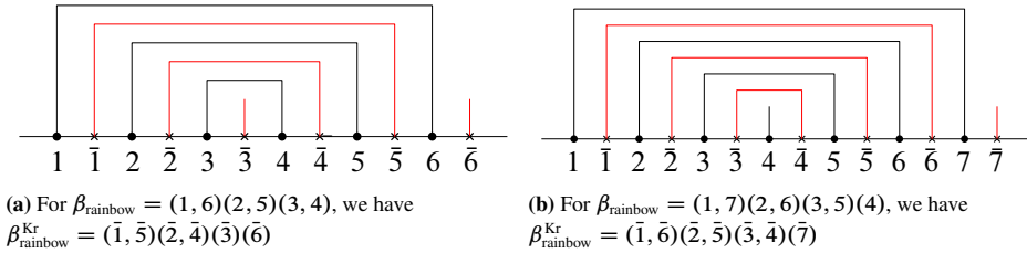
Figure 7. Examples for the rainbow partition \beta_{\text{rainbow}} when n = 6, 7 and its Kreweras complement.
