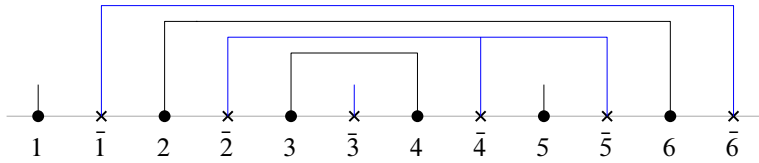
Figure 3. The Kreweras complement of \alpha = \{1\} \sqcup \{2, 6\} \sqcup \{3, 4\} \sqcup \{5\} is \alpha^{Kr} = \{1, 6\} \sqcup \{2, 4, 5\} \sqcup \{3\} .
