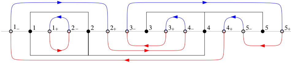
Figure 4. A meandric system generated by the geodesic permutations (in black) \alpha = (1, 2)(3, 4, 5) and \beta = (1, 2, 4)(3)(5) . The two loops (blue and red together) with arrows are formed by the action of \alpha^{-1}\beta .
