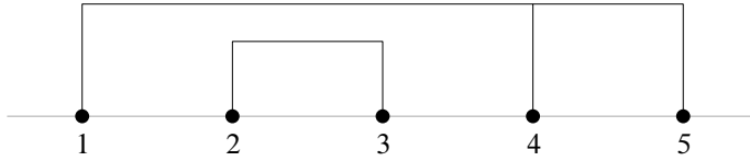
Figure 1. A non-crossing partition.
