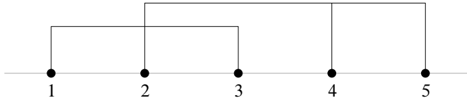
Figure 2. A crossing partition.
