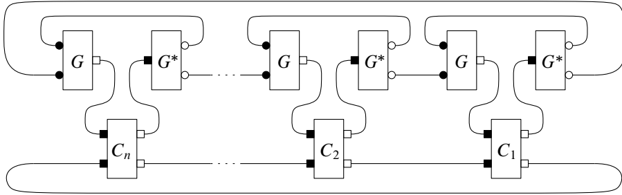
Figure 10. The diagram corresponding to \text{Tr}[Z_0 Z^{n-1}] .
