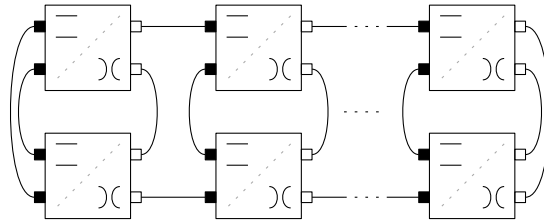
Figure 14. The diagram for \text{Tr}[\omega_l Z^{n-1}] . Each row contains (n - 1) boxes corresponding to the Choi–Jamiołkowski matrix of the map \Psi .
