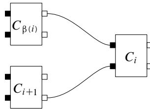
Figure 11. Connecting the Choi–Jamiołkowski matrices C_i by the permutation \beta and \gamma , where \gamma(i) = i + 1 .
