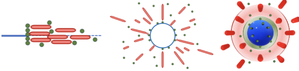
Figure 2: Reductions to 1–dimensional (left), 2–dimensional radially symmetric (middle), and 3–dimensional radially symmetric (right) geometries, respectively. The green dots represent the P proteins, while the red rods represent the S proteins.
