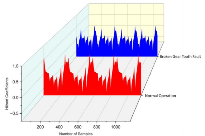
Fig. 6. A comparative HT analysis of air gap magnetic flux density of the PMSG for normal operation vs broken gear tooth faults
