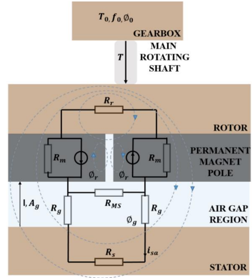
Fig 1. Magnetic Equivalent Circuit of PMSG coupled with a gearbox
