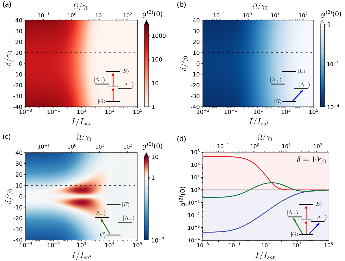
FIG. 2. Dependence of the color-blind intensity correlation g^{(2)}(0) on the laser intensity I and molecular detuning \delta . In (a) the laser is tuned to the two-photon resonance ( 2\omega_{\text{las}} = 2\omega_0 ), which leads to bunched emission. In (b) the laser excites resonantly the superradiant state |\Lambda_{-}\rangle ( \omega_{\text{las}} = \omega_0 - \Lambda ) giving raise to antibunched emission. In (c) the laser is tuned to the transition frequency of the subradiant state |\Lambda_{+}\rangle ( \omega_{\text{las}} = \omega_0 + \Lambda ) and g^{(2)}(0) shows a more complex dependence on the laser intensity and molecular detuning. In (a)–(c), color blue represents antibunched emission [ g^{(2)}(0) < 1 ], red bunched emission [ g^{(2)}(0) > 1 ], and white Poissonian statistics [ g^{(2)}(0) = 1 ]. Cuts of the results in (a)–(c) for \delta = 10\gamma_0 (along the dashed-black lines) are plotted in (d), where the red line corresponds to a laser tuned to the two-photon resonance, the blue line is obtained for a laser tuned to the superradiant state and the green line corresponds to a laser tuned to the subradiant state. In (d), red and blue shaded background correspond to bunched and antibunched statistics, respectively. The insets illustrate the different laser detunings considered. The dipole-dipole coupling is fixed as V = -20\gamma_0 and the combined Debye-Waller/Franck-Condon factor as \alpha = 0.3 .
