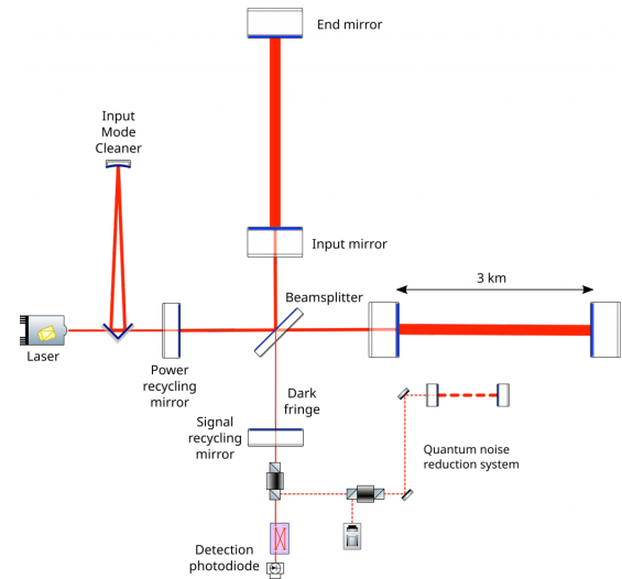
Figure 1: Schematic representation of the optical layout of the Advanced Virgo interferometer [4]
