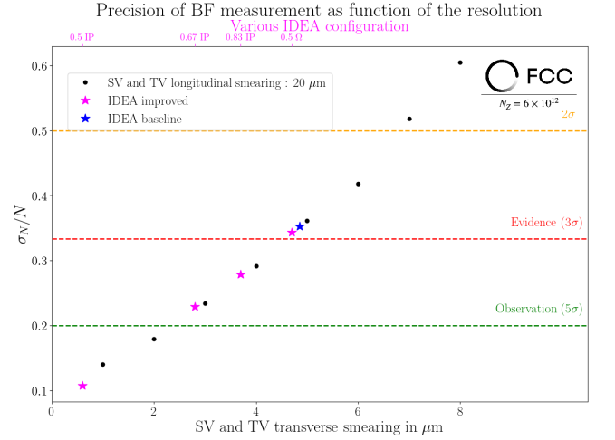
Figure 7: Precision of the B^0 \rightarrow K^{*0} \tau \tau branching fraction measurement at FCC- ee as function of the vertexing performances.
