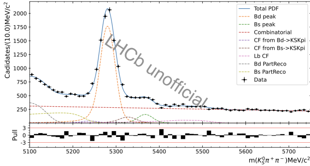
Figure 1: Mass fit spectrum for a K_S^0 \pi^+ \pi^- 2018 subsample. Colored curves exhibit the contribution of the participating decay channels and background.
