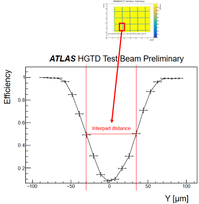
Figure 12: One example of interpad distribution and distance
