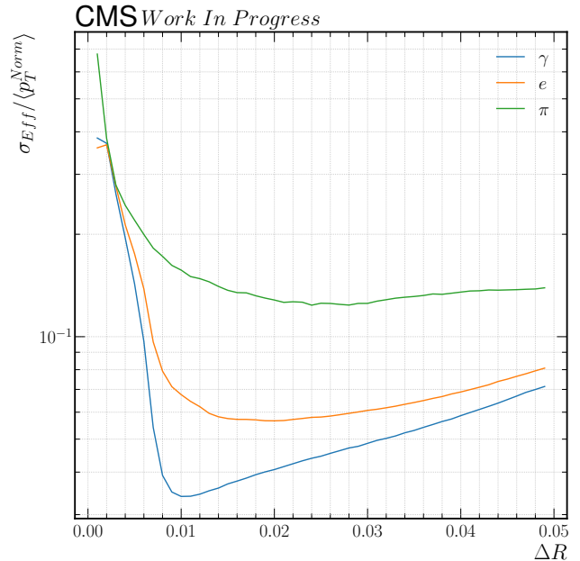
Figure 8: Energy resolution of the 3D clusters as a function of the clustering radius. Optimal clustering radii are given by \Delta R \sim 0.01 and \Delta R \sim 0.02 for electromagnetic and hadronic showers, respectively.
