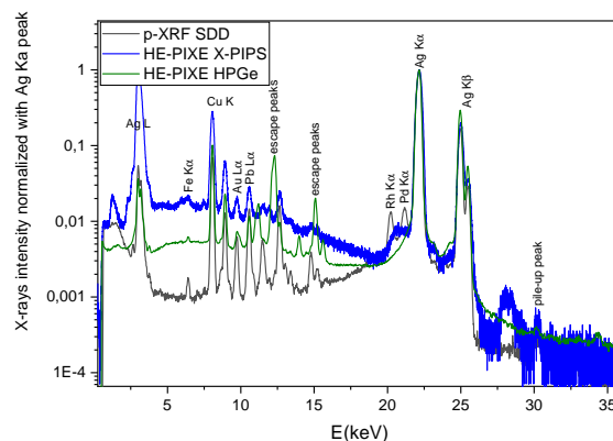
Figure 5: High energy spectrum - 1/4 d ecu - Charles X
