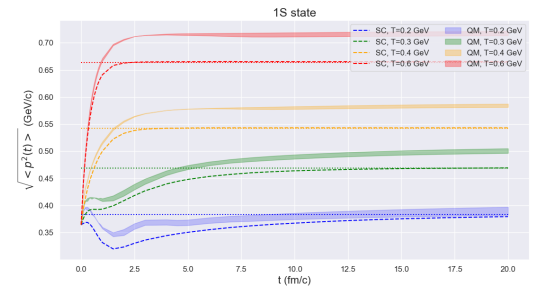
Figure 2: Time evolution of root mean squared momentum for various QGP temperatures with an initial 1S state. The dotted lines refer to the stationary values expected from Gibbs-Boltzmann distribution, i.e \sqrt{\langle p^2 \rangle_{\infty}} = \sqrt{MT/2} .
