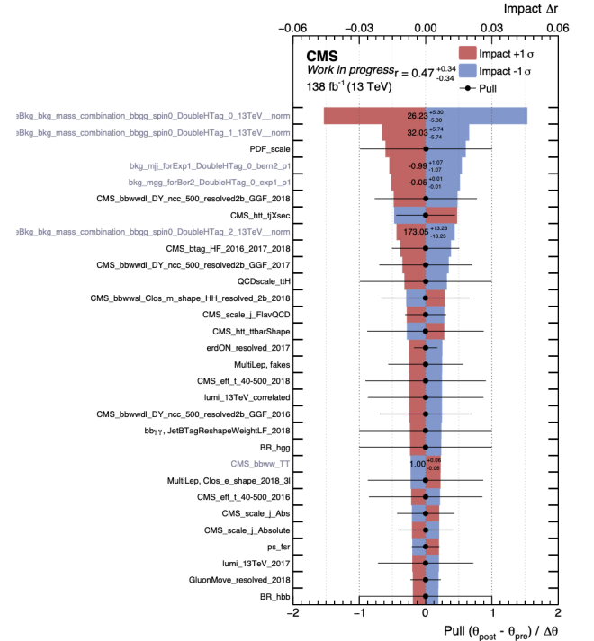
Figure 5: Pulls (black lines) and impacts (blue and red areas) of the 30 systematic uncertainties with the highest ranking for the combined expected (blinded) result for a mass M_X = 500 GeV
