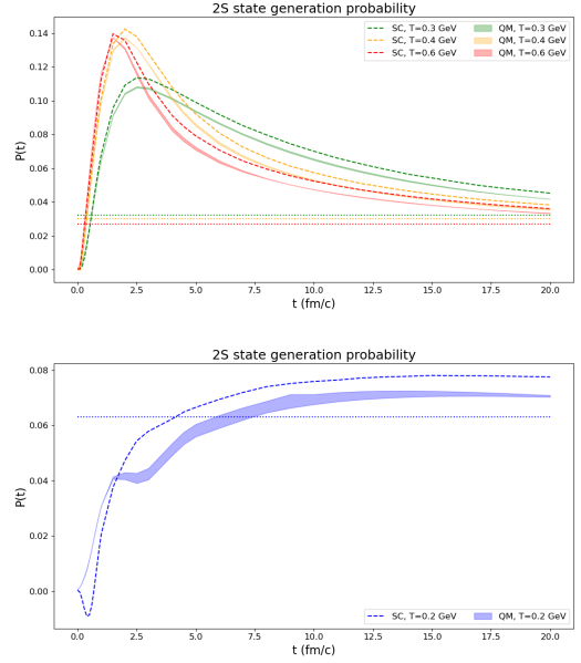
Figure 4: Generation probability of 2S state for T = [0.3, 0.4, 0.6] (GeV) (Top) and T = 0.2 (GeV) (Down). Dotted lines are the equilibrium values expected from Gibbs-Boltzmann distribution.
