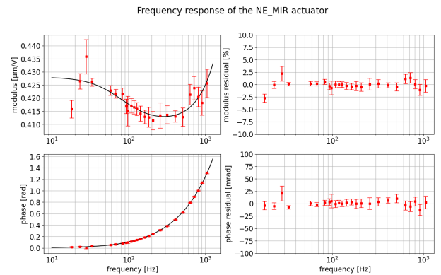
Figure 2: Example of calibration result for the actuator response of the NE mirror electromagnetic actuator. The top plots are the modulus and the bottom ones the phase of the actuator response. The left side represent the measurement result with the red points the data and the black line the fitted model. The right side is the residuals of the model.
