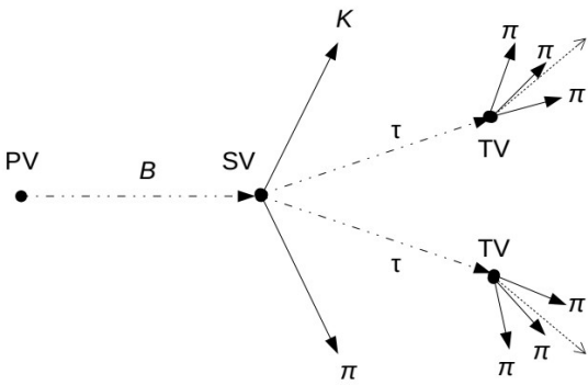
Figure 4: B^0 \rightarrow K^{*0}\tau\tau with \tau \rightarrow \pi\pi\pi\nu decay topology.
