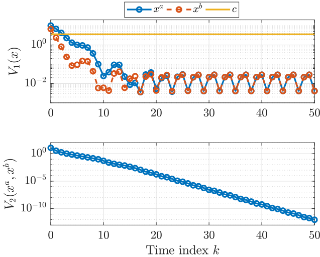
Fig. 5. Top: Lyapunov function V_1 along the trajectories x^a (solid blue) and x^b (dashed red). Bottom: Incremental Lyapunov function V_2 evaluated along x^a - x^b .
