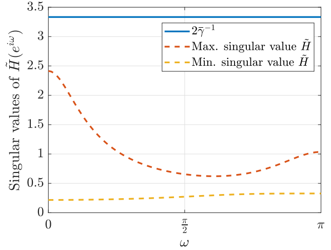
Fig. 2. The singular values of the transfer function matrix \tilde{H}(e^{i\omega}) as a function of the frequency \omega (dashed lines) and the threshold 2\bar{\gamma}^{-1} (solid line).
