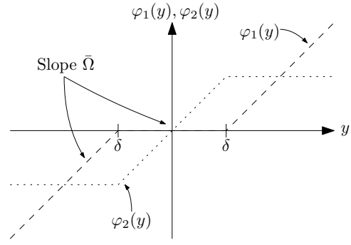
Fig. 1. Graph of \varphi_1 (dashed) and \varphi_2 (dotted) with deadzone/saturation length \delta and slope \bar{\Omega} .
