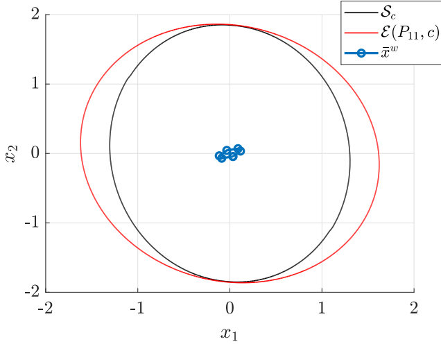
Fig. 4. The steady-state state trajectory \bar{x}^w (blue), the level set V_1(x) = c (black), and the ellipsoid \mathcal{E}(P_{11}, c) .
