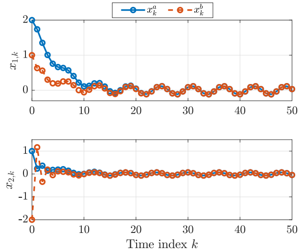
Fig. 3. Time response for initial conditions x_0^a (solid blue) and x_0^b (dashed red) for the input w_k = \cos(k\pi/3) .
