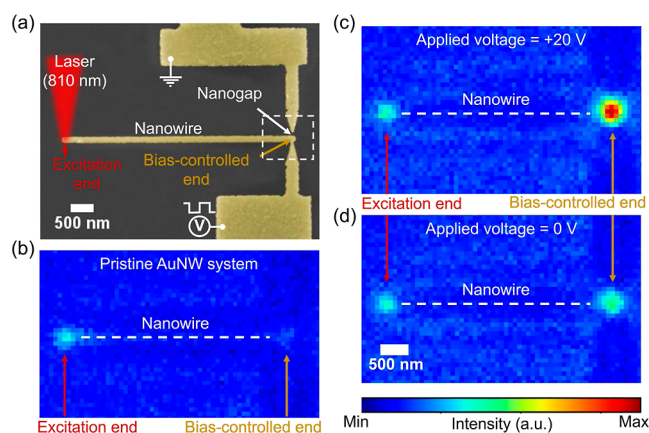
Figure 1. Overview of the AuNW system and its operation: (a) Device configuration seen from a colorized SEM image of a typical AuNW system. A tightly focused laser excitation at the left end of the AuNW is used to launch a propagating surface plasmon at the pump wavelength (810 nm). The distal end is electrostatically controlled by a tapered electrode placed at a 50 nm distance from the AuNW surface. (b) Spatial distribution of the N-PL on a pristine AuNW. The signal arises from the extremity directly excited by the focused laser as well as from the distal end via the mediation of a surface plasmon. (c,d) Same as in (b) for V = +20 V and V = 0 V, respectively, after electrical activation of the nanogap. A localized enhancement of the signal at the bias-controlled end is readily seen with applied bias. The dashed white line represents the long axis of the nanowire.
