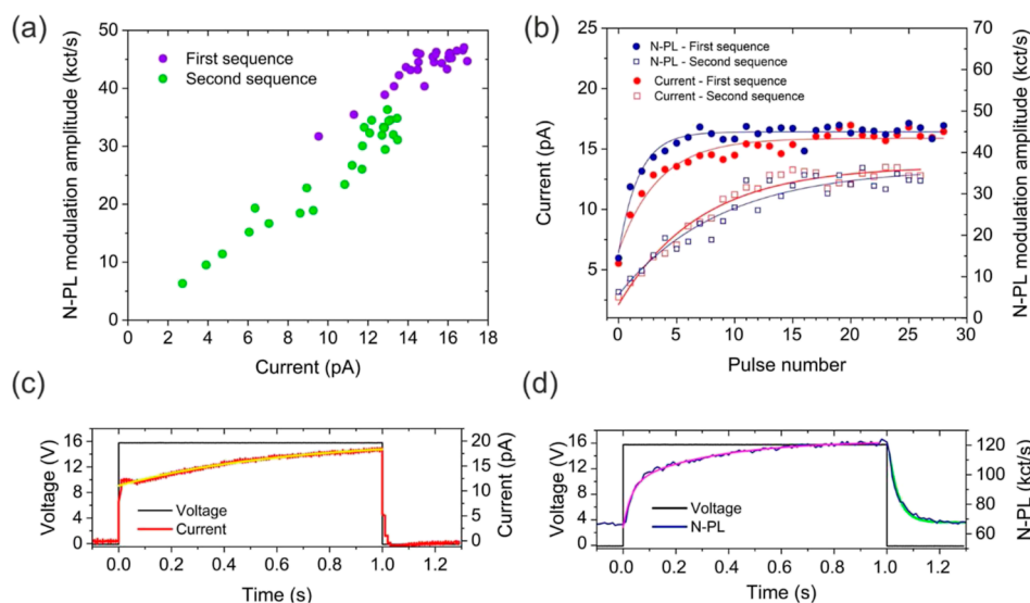
Figure 3. (a) N-PL modulation amplitude plotted against the electric current, I_g , for the two positive bias sequences shown in Figure 2c. (b) Pulse-to-pulse evolution of the N-PL modulation amplitude and I_g amplitude for the two positive bias sequences. Solid lines are fits of the data with a simple capacitor-like function. (c,d) I_g and N-PL intrapulse dynamics averaged over 29 consecutive positive bias pulses. A spurious 25 Hz component has been filtered out from the N-PL signal. I_g is fitted with a capacitor model in the slow-growth region to extract the time constant (yellow solid line). N-PL is best fitted with a double exponential after the leading bias edge (purple solid line). However, the decaying tail after the falling edge is well reproduced as a simple picture of a discharging capacitor (green solid line).
