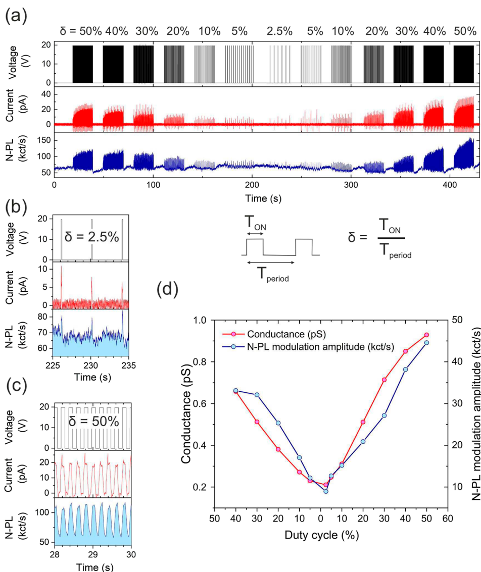
Figure 5. (a) Time series of N-PL and electric current, I_g , response under 100 ms bias pulses with +20 V amplitude and varying duty cycle \delta = T_{\text{ON}}/T_{\text{period}} shown in the inset at the top. (b,c) Zoomed snapshots of time series for duty cycles \delta = 2.5\% and \delta = 50\% . (d) N-PL modulation amplitude and average conductance of the nanogap during the bias pulse with varying duty cycles of applied bias pulses calculated from different bias pulse sequences of time series presented in (a).
