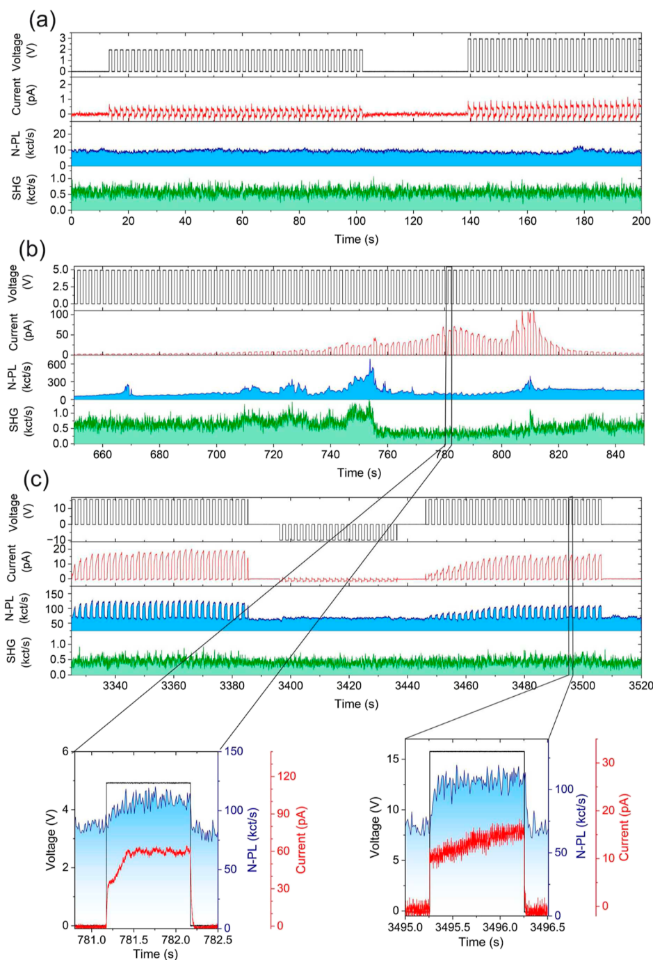
Figure 2. (a–c) Snapshots of the time series showing the evolution of modulation amplitudes in spatially filtered N-PL and second-harmonic generation (SHG) from the bias-controlled end of AuNW and electric current, I_g , passing through the nanogap under electrostatic bias pulse sequences. Single-pulse details of the time traces are shown at the bottom.
