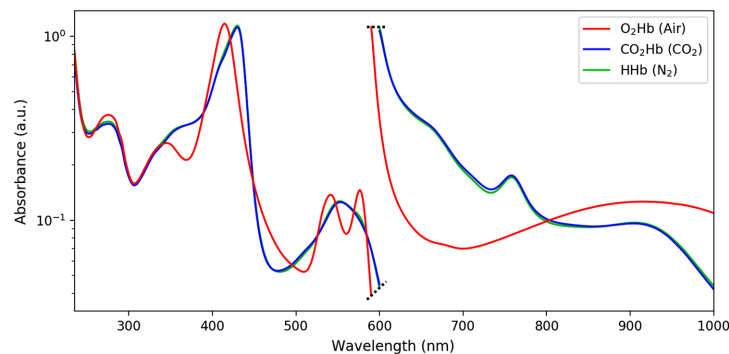
Fig. 3 Measured absorption spectra of diluted lysed blood tonometered with \text{O}_2 , \text{N}_2 , or \text{CO}_2 . The vertical scale is arbitrary, data were scaled for representation and corresponds to two different dilution ratios of 1:1000 for the UV–Vis 235 to 600 nm range (left) and 1:10 for the Vis–IR 600- to 1000-nm range (right) (ranges are 235 to 590 nm and 590 to 1000 nm for air-equilibrated solutions). The black dashed line separates the UV–Vis from the Vis–IR measurements.
