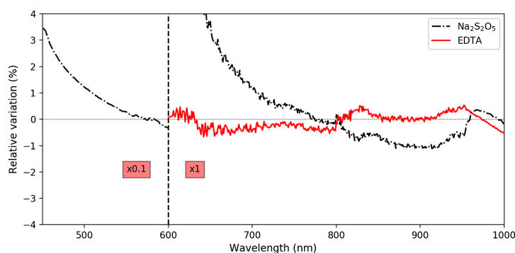
Fig. 6 Relative variations of the dilution medium absorption spectrum upon the addition of EDTA (0.61 mM) or sodium metabisulfite (2.0 mM). The left side is multiplied by 0.1 ( \sim 10\% of relative variation for sodium metabisulfite at 500 nm).
