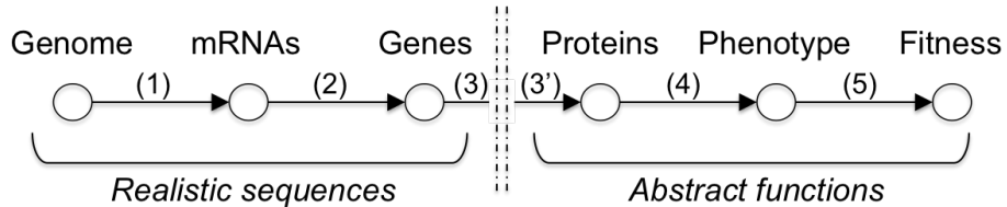
Figure 4: Overview of the Genotype-to-Phenotype map in aevol. Genomes are decoded into a phenotype through a multi-step process that first decodes the genome sequence to identify the genes (steps 1 and 2), then decodes the gene sequence to compute the protein functions (step 3 and 3'), the phenotype (step 4) and ultimately the fitness of the organism (step 5). See main text for details.
