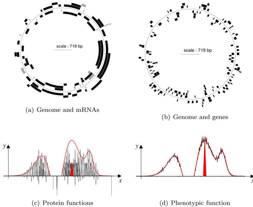
Figure 5: Overview of an aeol wild-type. Top: sequence level (genome, RNAs and genes). The double-stranded genome is represented by a circle (thin line). Black arcs represent mRNAs (a) and genes (b) on each strand (grey arcs represent non-coding RNAs and non-functional genes respectively). Note the presence of polycistronic sequences. Bottom: environmental target (red curve) and functional levels (proteins and phenotype, in black) with one specific function highlighted in red. (c) Each triangle corresponds to a protein function which parameters are decoded from the sequence of a gene. Note the presence of function-activating/repressing proteins (positive/negative triangles respectively). (d) Organism's phenotype resulting from the sum of all protein functions. To illustrate the effect of gene duplication, one protein function has been highlighted in red on panel (c). This protein is not active enough to fit the target. However, as the corresponding gene exists in three copies on the genome, the overall effect is amplified through dosage effect (red triangle on panel d), hence increasing the contribution of this protein on the y axis without changing the set of functions it contributes to on the x axis.
