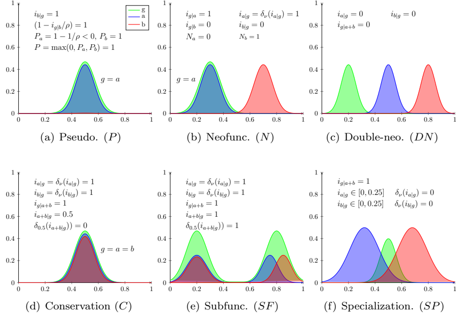
Figure 2: The canonical fates using the Gaussian representation. Note that in the case of SF and SP , i_{g|a+b} is not exactly 1, but we assume that this is the case for the sake of simplicity. We assume thresholds \rho = 0.2 (relevant for P ) and \nu = 0.25 (mostly relevant for SP ). In (a), b has become a shape of height 0 and is considered as a pseudogene. In (e), SF can occur in two ways: a and b retain the same functions as g , but split their expression levels (left), or a and b split a portion of the functions of g (right).
