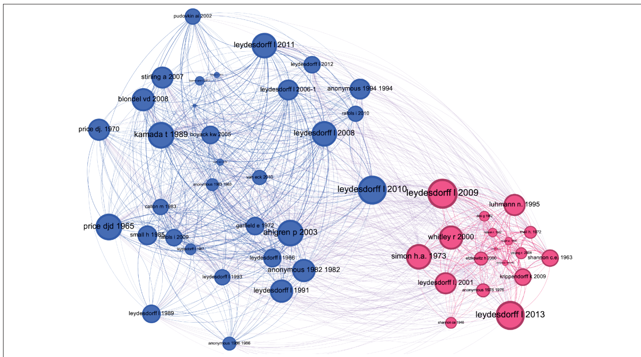
Figure 8. Leydesdorff's publication co-citation network
