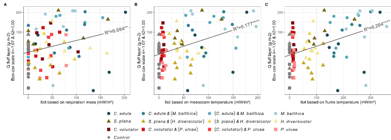
Figure 4 Fluff layer quantity ( Q_{fluff} [ g.m^{-2} ]) vs the different metabolic rate evaluation [ mW.m^{-2} ]: based on the measured respiration rate Itot_{respi} (A), the Itot with the mesocosm temperature Itot_{meso} (B) and the Itot with the flume temperature Itot_{flume} (C) and their regression line. Note that the y scale is Box-Cox transformed, and the models were made on transformed data.
