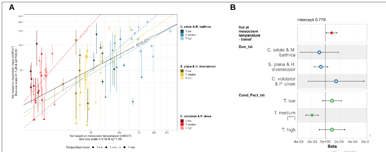
Figure 3 A: Itot_{respi} [ mW.m^{-2} ] vs Itot_{meso} , with standard deviation and its regression line for each duo (corresponding colours) and in grey for all data combined, the grey dotted line represents the identity relation. Note that the scales are Box-Cox transformed, and the regression lines were made on transformed data. B: ANCOVA results for Itot_{respi} transformed \sim Itot_{meso} transformed + Duo + Temperature. Filled dot are p-value \leq 0.1 and empty dot are p-value > 0.1 .
