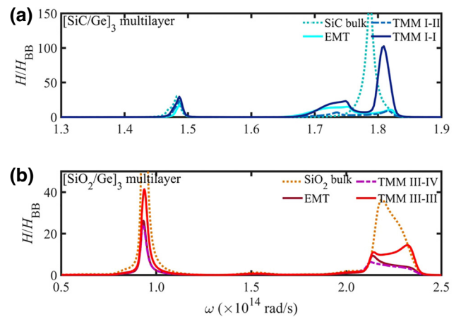
FIG. 4. Near-field spectral heat flux for different combinations of (a) SiC/Ge and (b) [\text{SiO}_2/\text{Ge}] multilayer samples. Spectral heat flux is normalized to that of the blackbody with H/H_{\text{BB}} . Results of bulk SiC and \text{SiO}_2 are also provided for comparison.
