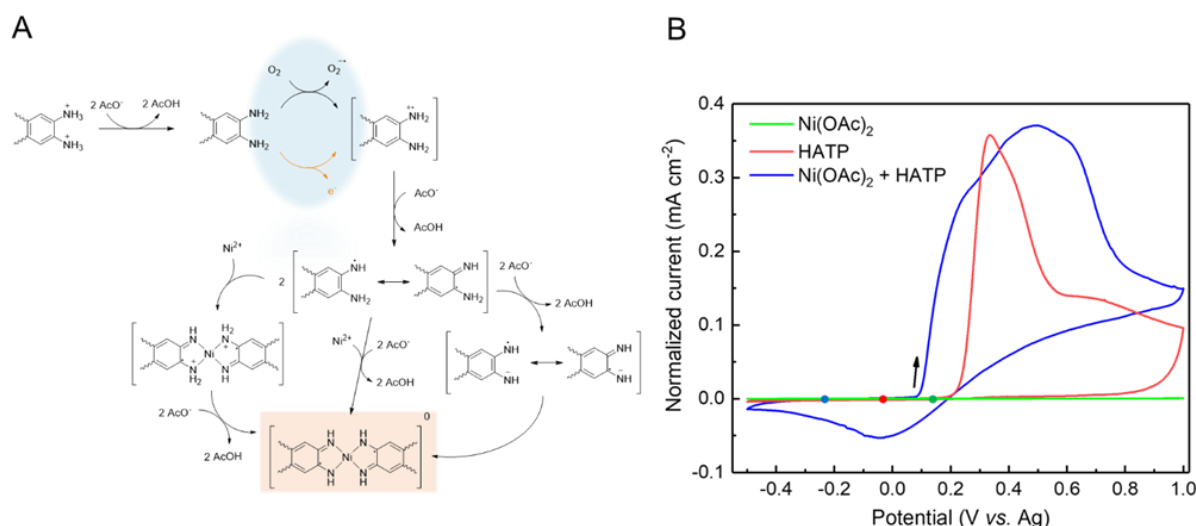
Figure 1. (A) The mechanism of Ni 3 (HITP) 2 synthesis implying initial HATP ligand chemical or electrochemical oxidation, followed by a series of acid-base and coordination reactions. (B) Cyclic voltammograms of individually containing Ni(OAc) 2 and HATP solutions, as compared to the Ni 3 (HITP) 2 precursors electrolytic bath, all acquired at a scan rate of 10 mV.s -1 on ITO working electrode.
