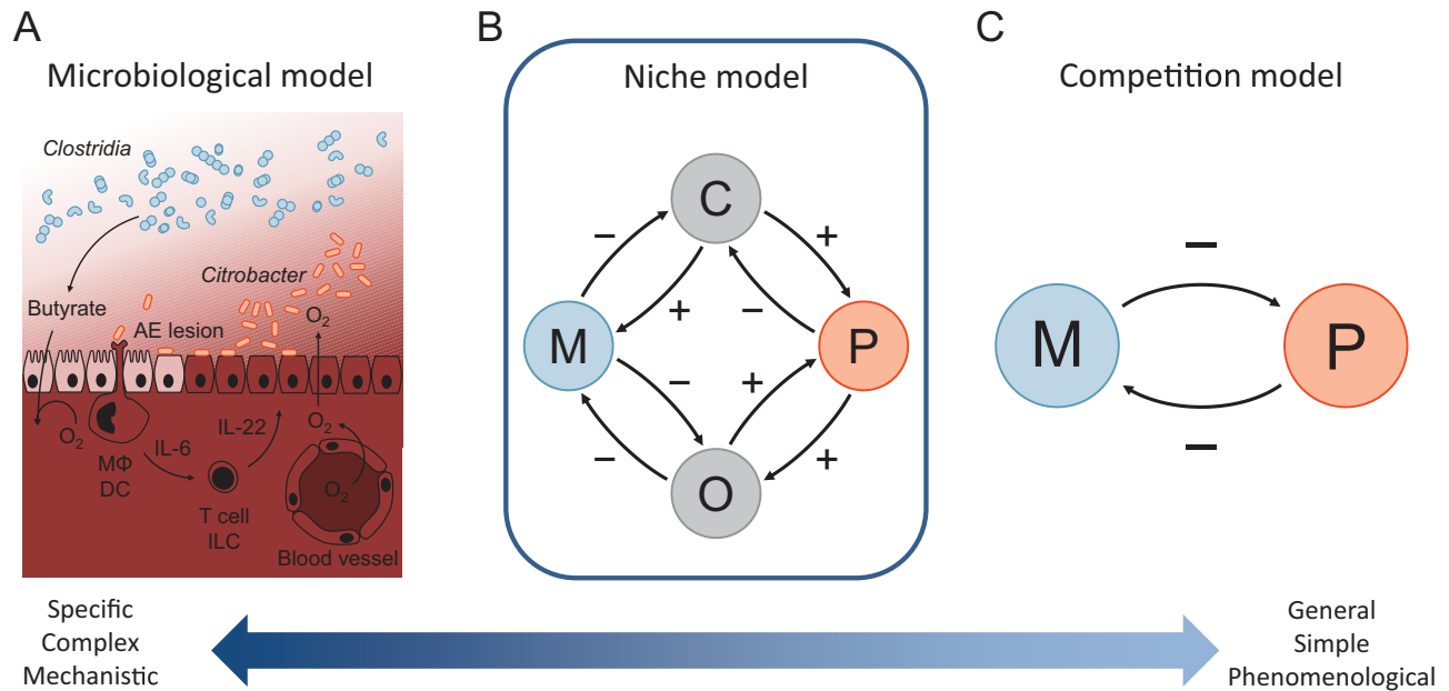
Figure 1: Continuum of modeling approaches. Gut community modeling approaches range from A , microbiological models that focus on specific genes, regulatory networks, and biochemical reactions, to B , resource-competition-based models that focus on population dynamics, environmental state variables, and their interactions using generalized ecological mechanisms instead of physiological mechanisms (our approach), to C , Lotka-Volterra models of two-species competition where environmental parameters are implicit and do not affect competitive dynamics. Model A is specific to Citrobacter rodentium (Rivera-Chávez et al. 2016, 2017), while models B and C are general to many enteric pathogens. Consistent with model variables, M and P respectively represent the abundances of anaerobic mutualists and pathogens, C represents shared carbon substrate, and O represents pathogen-preferred electron acceptors.
