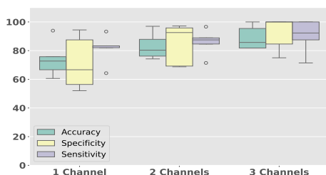
Figure 4: Drugs TdP-risk classification performance using a different number of modalities based on the voting classifier with Random-Forest, K-Nearest-Neighbors, Gaussian Naive Bayes and Linear Discriminant Analysis.
