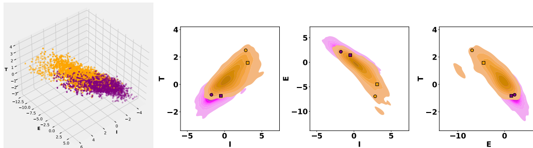
Figure 3: Left: scatter plot of all drugs in the 3D latent space. Right: Kernel density distribution of drugs for each pairwise combination of latent channels. Unsafe drugs are in orange; safe drugs are in purple.
