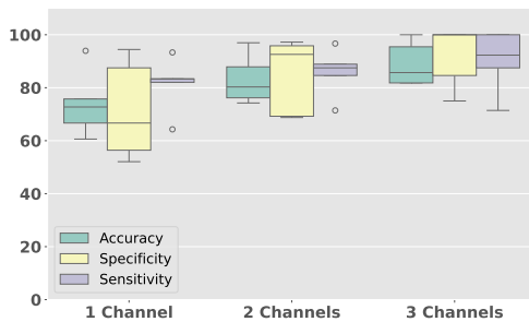
Figure 4: Drugs TdP-risk classification performance using a different number of modalities based on the voting classifier with Random-Forest, K-Nearest-Neighbor, Gaussian Naive Bayes and Linear Discriminant Analysis.
