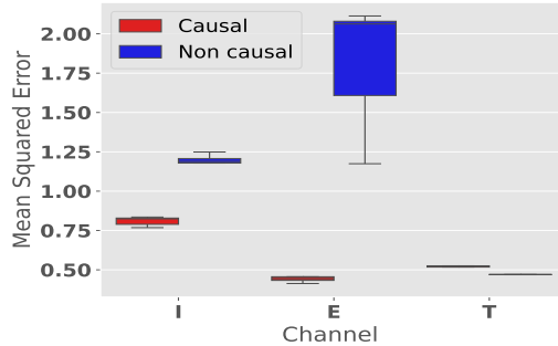
Figure 2: Mean squared errors per channel.
