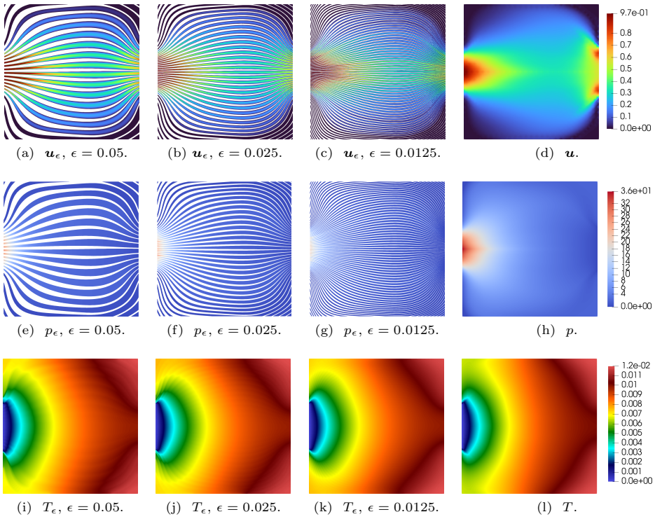
Fig. 24: The first three columns, from left to right, depict the velocity, pressure, and temperature fields obtained by solving the Stokes equations on a 2000 \times 2000 fine mesh for the upscaled structures with various \epsilon , cf. Fig. 23. The fourth column displays the homogenised velocity, pressure, and temperature fields acquired by solving the homogenisation equation on a 50 \times 50 coarse mesh. For comparison, the pressure fields obtained by the full-scale simulations are normalised by a multiplicative factor \epsilon^2 and the legend bar range is rescaled based on the homogenised model.
