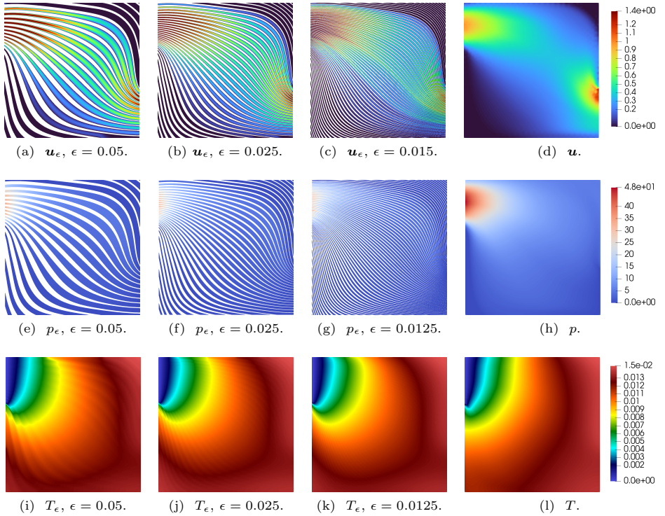
Fig. 30: The first three columns, from left to right, depict the velocity, pressure, and temperature fields obtained by solving the Stokes equations on a 2000 \times 2000 fine mesh for the upsampled structures with various \epsilon , cf. Fig. 29. The fourth column displays the homogenised velocity, pressure, and temperature fields acquired by solving the homogenisation equation on a 50 \times 50 coarse mesh. For comparison, the pressure fields obtained by the full-scale simulations are normalised by a multiplicative factor \epsilon^2 and the legend bar range is rescaled based on the homogenised model.
