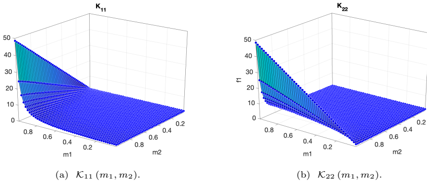
Fig. 6: Linear interpolation of \mathcal{K}_{11} and \mathcal{K}_{22} .
