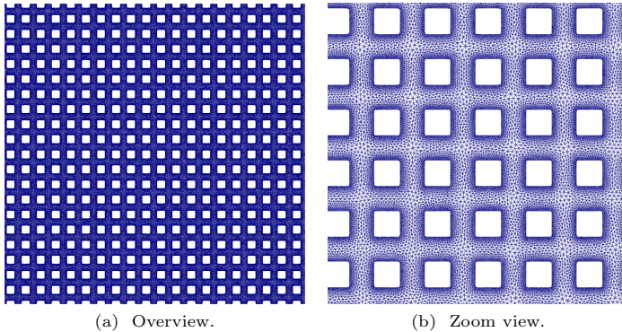
Fig. 16: A snapshot of the body-fitted mesh representing the fluid subdomain \Omega_{\epsilon,f} , derived from the initial guess where \epsilon = 0.05 .
