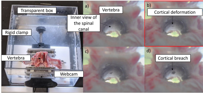
Fig. 5. On the left, we can see the setup; a webcam is filming the inside of the spinal canal. The right mosaic shows the deformations and bone penetration within the vertebral column while using the threaded instrument. There is no breach in the image (a); the image highlighted in red (b) denotes the moment the tool begins to exit the bone and enter the spinal canal. In images (c) and (d), we can see a progression of the tool through the cortical bone.
