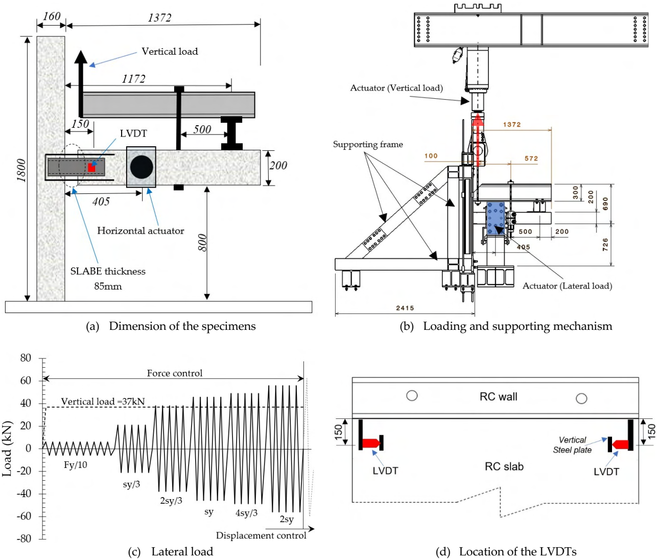
Figure 2. Dimensions and test setup (Dimensions in mm)
