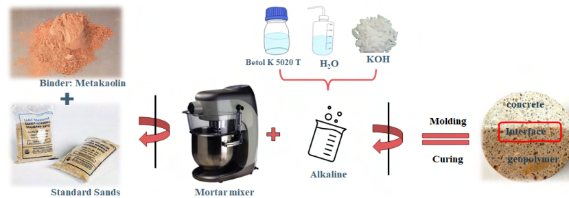
FIGURE 1. Geopolymer Mortar Preparation Flowchart
