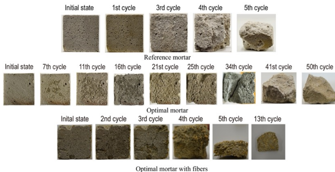
FIGURE 6. Effect of \text{Na}_2\text{SO}_4 solution on the aspect of the different mortars after curing time of 1 month.
