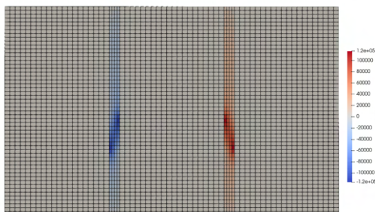
FIGURE 9. Shear stress distribution in the joint (left) and damage value (right) for a load of 4000 N.
