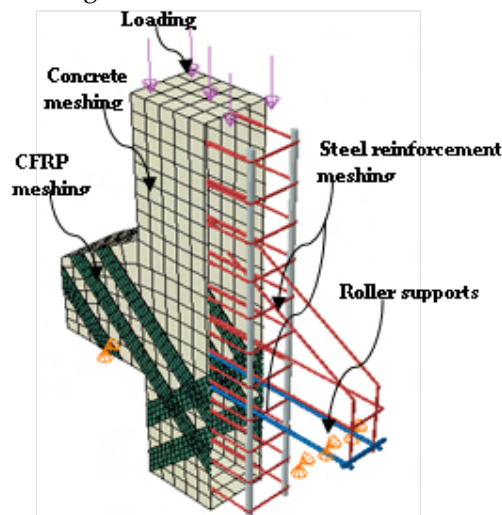
FIGURE 4. Meshing of concrete element, steel reinforcement, and CFRP strips
