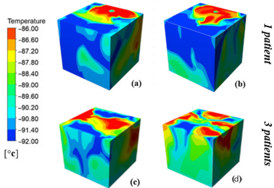
Figure 4. Distribution of temperatures inside the cryotherapy chamber when occupied by one person (a,b) and then three people (c,d), respectively, at t = 2 min and t = 3 min.
