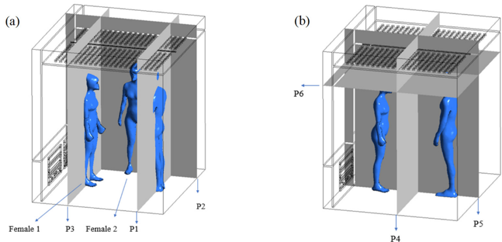
Figure 5. Plane positions. (a) Three planes passing through the human bodies; (b) Three other planes crossing the cabin through its symmetry planes.
