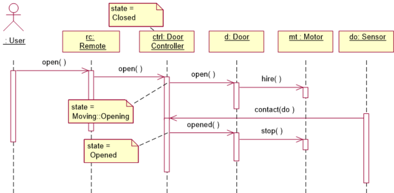
Figure 5. Opening Sequence diagram - garage door
