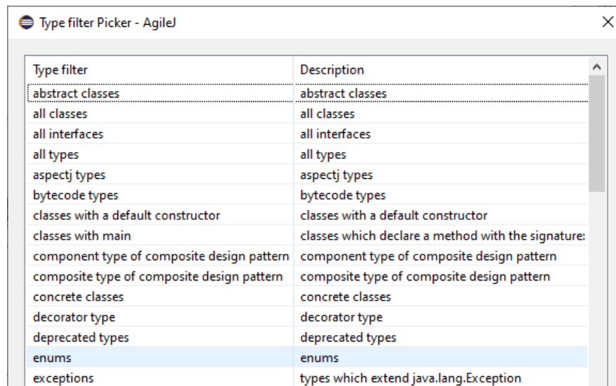
Figure 28. AgileJ filter process
