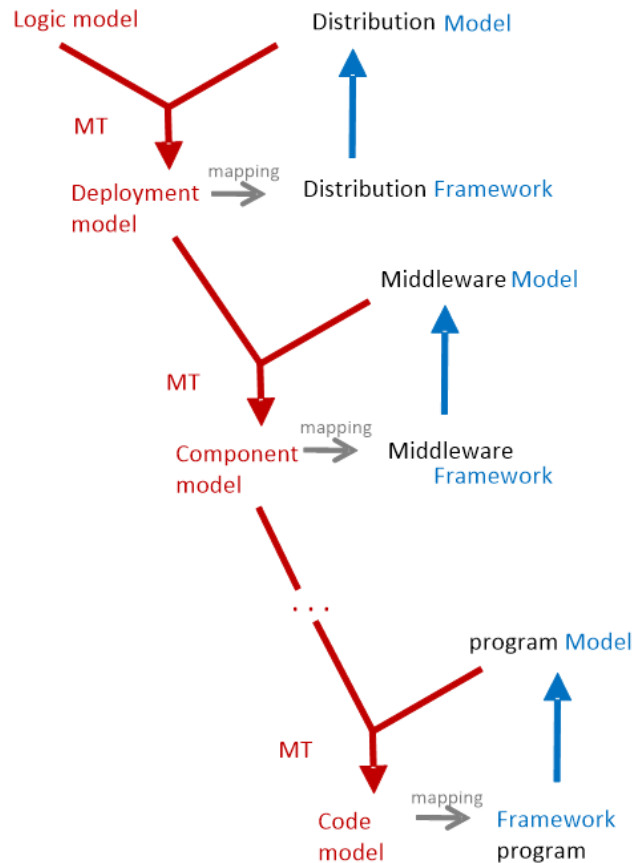
Figure 29. Mapping transformation process
