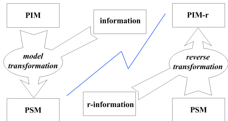
Figure 25. Reverse Model Transformation
