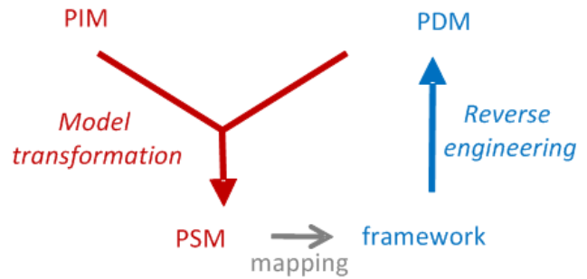
Figure 24. View of a mapping transformation
