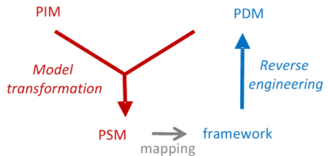
Figure 24. View of a mapping transformation
