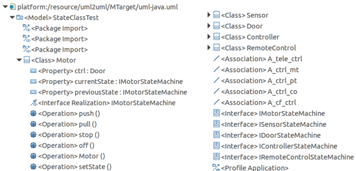
Figure 16. The Java elements generated for the garage door
