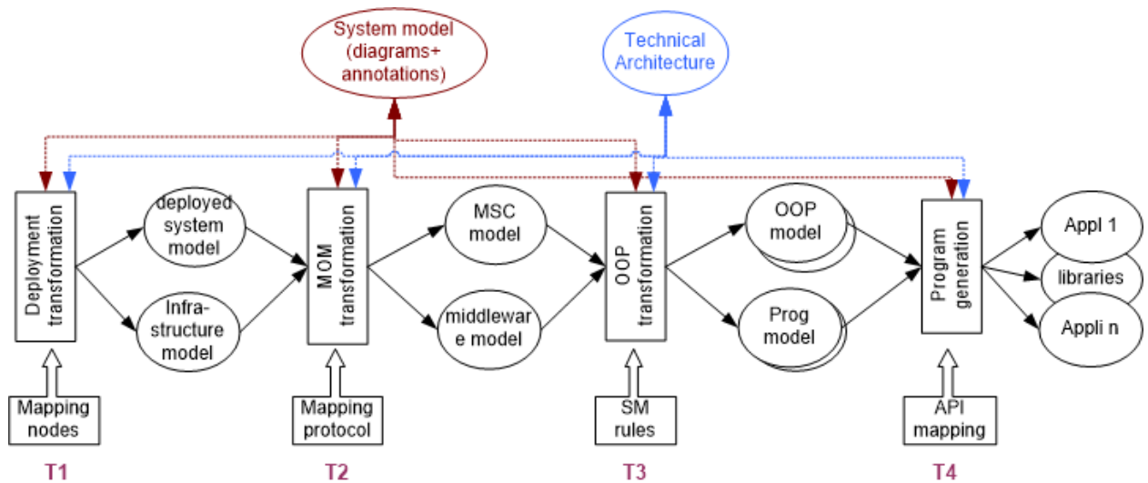
Figure 10. General transformation process
