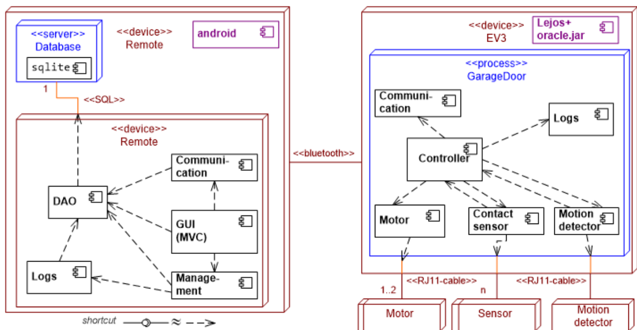
Figure 11. Deployment diagram - garage door
