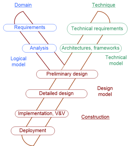
Figure 1. 2TUP Unified Process
