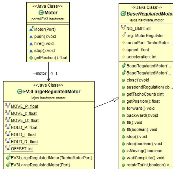
Figure 22. Class Mapping by Adaptation of the Motor Class
