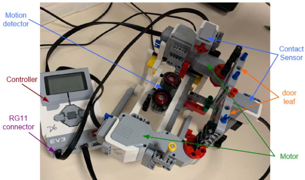
Figure 7. Lego prototype of the door system
