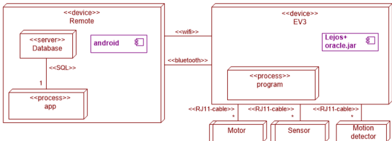
Figure 6. Technical Architecture - EV3 and app
