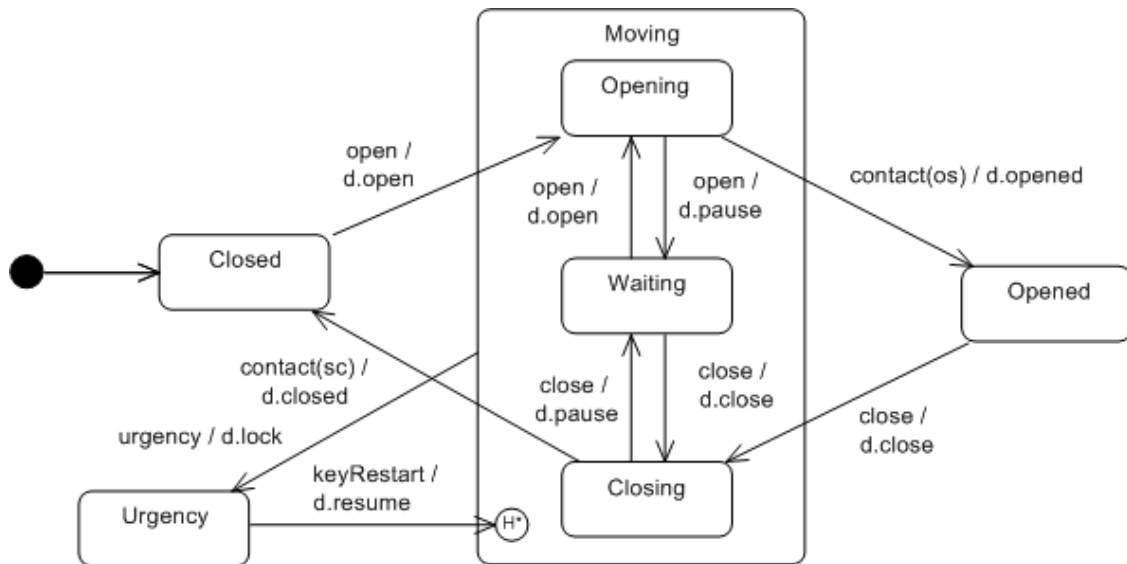
Figure 4. Door controller State diagram - garage door
