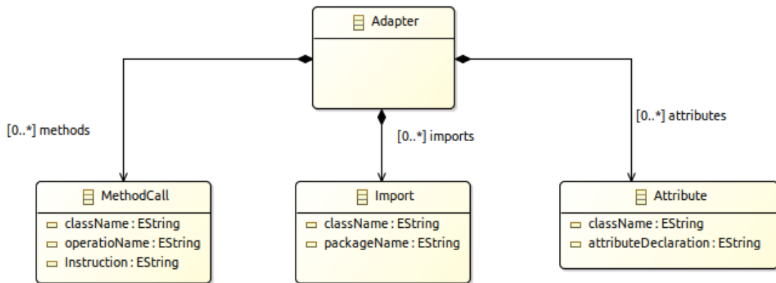
Figure 21. Adapter Pattern Model
