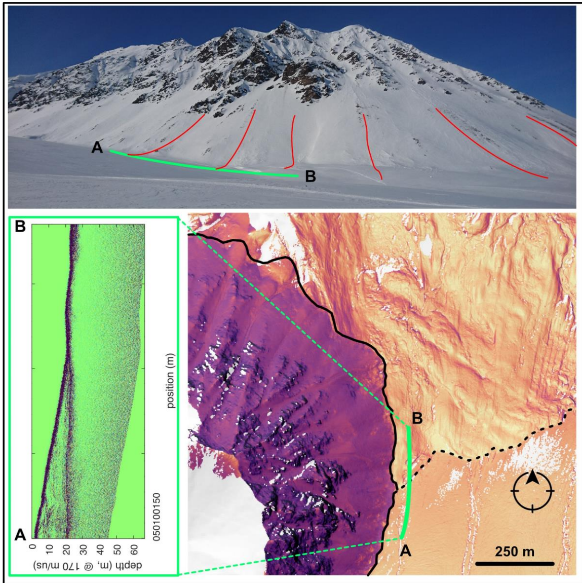
Figure 10: GPR transect along the glacier flow to identify the glacier front where ice thickness vanishes.
