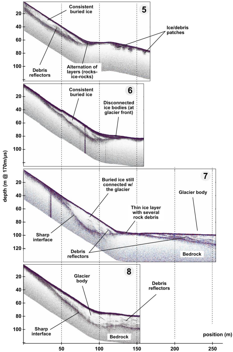
Figure 6: B-scan radargrams collected along transects 5 to 8, closest to the current glacier position. 149 deepest and high amplitude, interface is associated with the ice-bedrock boundary.
