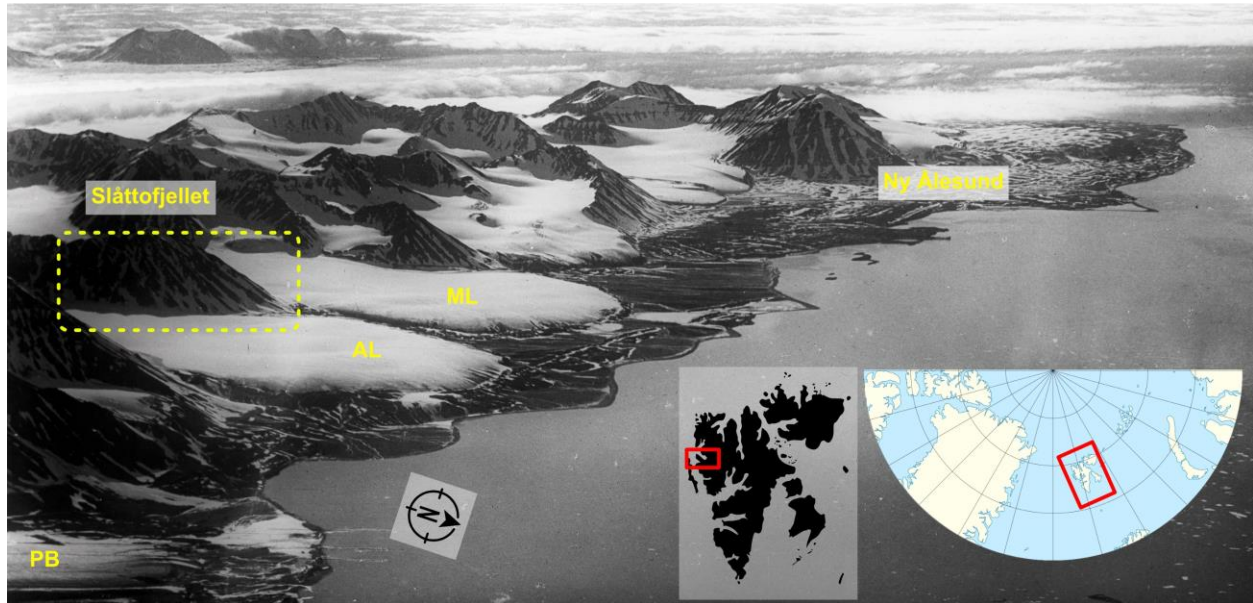
Figure 1: Historical aerial photography illustrating the maximum post-Little Ice Age extent of Brøggerhalvøya glaciers in 1923. Austre Lov'enbreen (AL) is surrounded by Midtre Lov'enbreen (ML, background) and Pedersenbreen (PB, foreground). The dashed square highlights the area of interest, in the slopes where AL and ML were once connected. Image in the public domain available from Wikimedia Commons.
