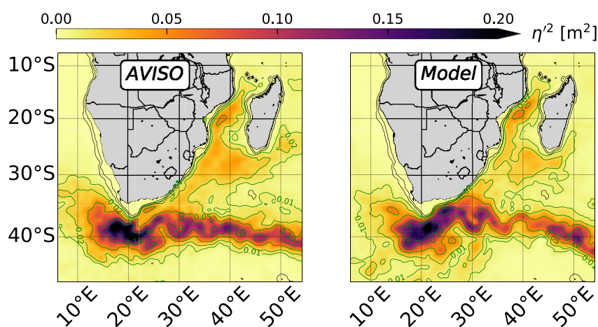
Figure A1. Observed and modeled mesoscale variability at the surface in the Agulhas Current system. \eta variance ( \eta'^2 ) [ \text{m}^2 ] performed from (a) satellite altimetry data (AVISO) and (b) a numerical simulation ( dx \sim 7.5 km). Green contours denote isolines of \eta variance and black contours denote 300 and 1,000 m isobaths.
