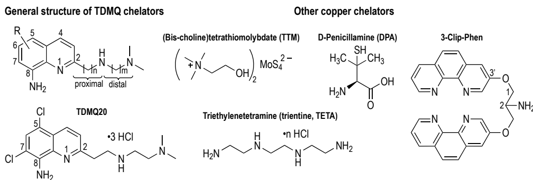
Figure 1. Structures of TDMQ specific Cu(II) chelators, and of some other Cu chelators considered for antiangiogenic properties.
