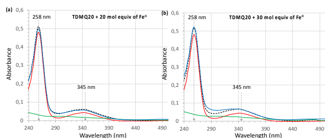
Figure 3. UV-visible spectra of TDMQ20 20 \mu\text{M} alone (red trace) or after addition of (a) 20 mol equiv or (b) 30 mol. equiv. of \text{Fe}(\text{SO}_4)_2(\text{NH}_4)_2 \cdot 6 \text{H}_2\text{O} , corresponding to 400 or 600 \mu\text{M} , respectively) (blue trace). The dashed black traces stand for the arithmetic addition of the spectrum of TDMQ20 + spectra of \text{Fe}(\text{SO}_4)_2(\text{NH}_4)_2 \cdot 6 \text{H}_2\text{O} , (a) 400 or (b) 600 \mu\text{M} alone. The spectra of \text{Fe}(\text{SO}_4)_2(\text{NH}_4)_2 \cdot 6 \text{H}_2\text{O} alone (a) 400 or (b) 600 \mu\text{M} (green traces), are given for comparison.
