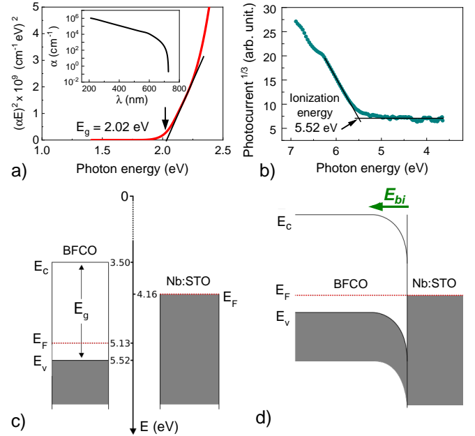
FIG. 6. (a) Tauc plot for a BFCO film grown on a Nb:STO substrate. Inset: The absorption coefficient vs wavelength as obtained from ellipsometry measurements (see Fig. S3 in the Supplemental Material [49]). (b) Photocurrent plot, obtained by photoemission spectroscopy, used to determine the ionization energy. (c) Energy level diagram of the BFCO/Nb:STO structure based on results from (a) and (b). Expected electronic band structure of BFCO/Nb:STO interface. A built-in electric field ( E_{bi} ) pointing from the Nb:STO towards the BFCO is expected within the space charge region.
