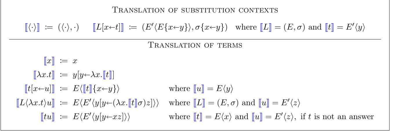
Fig. 7. The translation from \lambda_{\text{ovsc}} to \lambda_{\text{oxpos}} .
