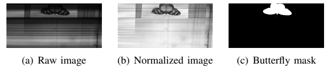
Fig. 5. Butterfly detection
