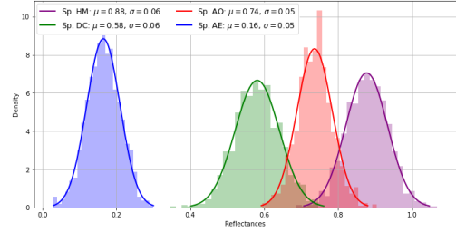
Fig. 4. Gaussian distribution in Spectral Layer 154.
