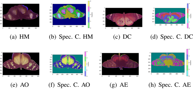
Fig. 3. Spectral clusters (Spec. C.) of butterfly species
