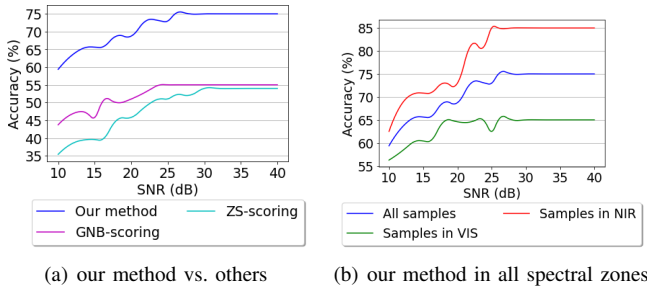
Fig. 6. Accuracy classification given multiple SNR on test images
