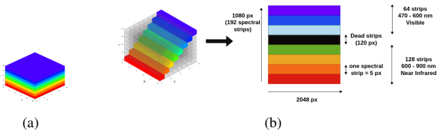
Fig. 1. Captured HSI content from (a) a conventional and (b) a spatio-spectral camera (structure of our camera).
