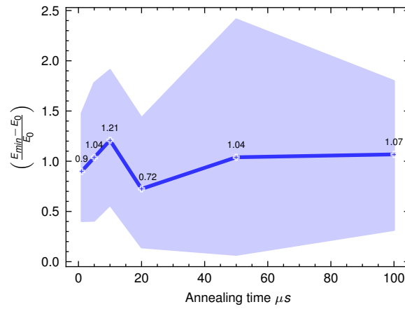
Fig. D5: Overall Effect of annealing time on QA performance, measured as the mean relative deviation from the ground state \left(\frac{E_{min} - E_0}{E_0}\right) for cumulative instances with a OS = 0.1 and all sizes (3,4,5,6,7 and 8 non-dummy activities).
