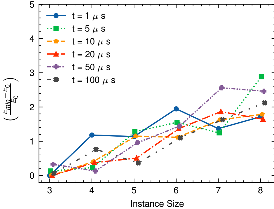
Fig. 15: Mean Effect of annealing time on QA performance, measured as the mean relative deviation from the ground state \left(\frac{E_{min}-E_0}{E_0}\right) for all instance types (OS = 0.1, OS = 0.5 and OS = 0.9).
