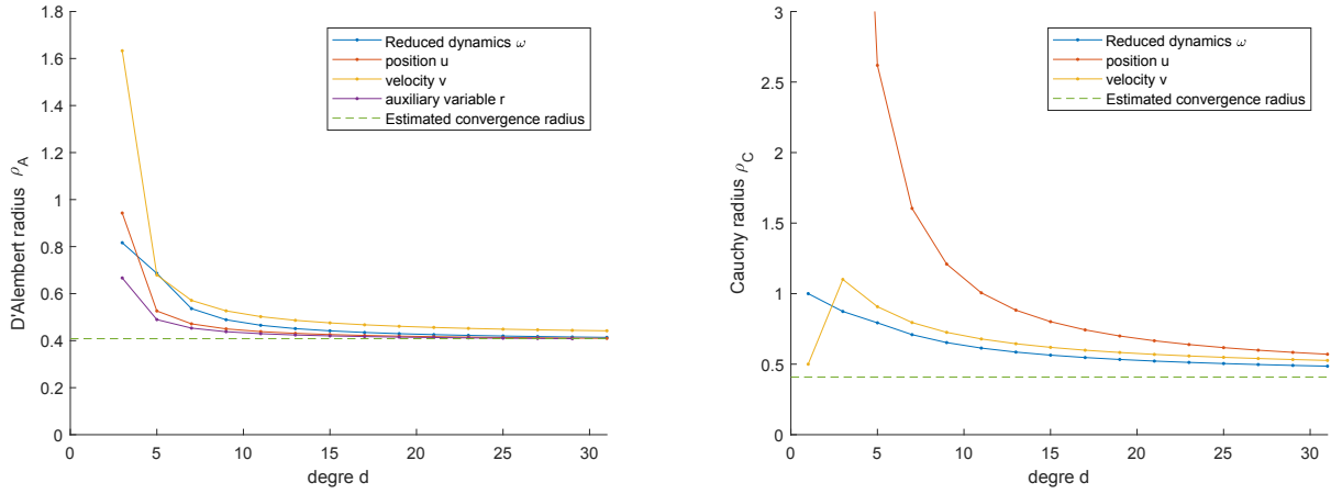
Figure 2: Left plot: Evolution of the d'Alembert coefficients as a function of the degree d (for \theta = 0 ). Right plot: Evolution of the Cauchy coefficients as a function of the degree d (for \theta = 0 ).
