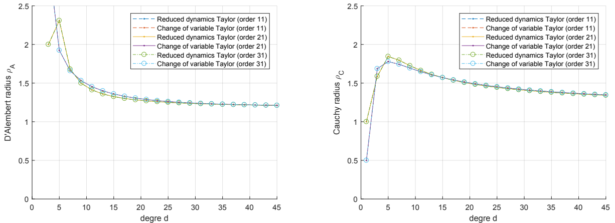
Figure 5: Left plot: Evolution of the d'Alembert radius of convergence \rho_A as a function of the degree d (for \theta = 0 ). Right plot: Evolution of the Cauchy radius of convergence \rho_C as a function of the degree d (for \theta = 0 ).
