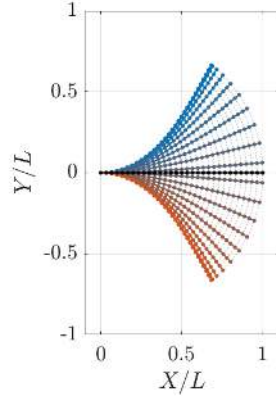
Figure 17: Vibration shape of the first mode of the cantilever beam at the quantitative validity limit amplitude of the normal form of degree 31
