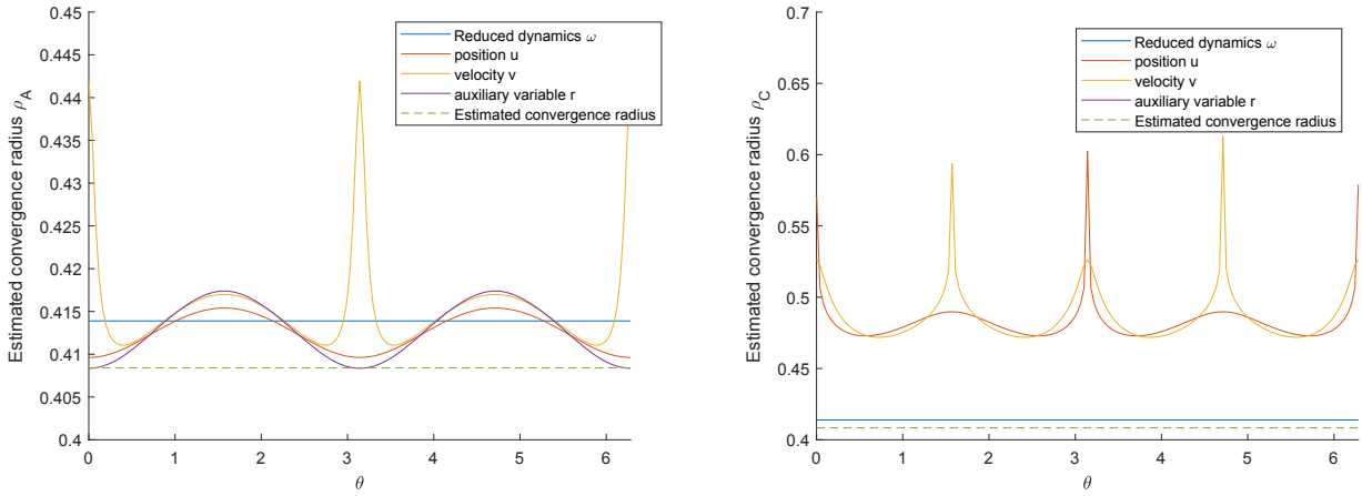
Figure 3: Evolution of the estimated convergence radius \rho_A and \rho_C as a function of the angle \theta (position along the period) for the different series of the reduced dynamics ( \omega = \theta ) and the change of variables ( u, v, r ). Left: d'Alembert coefficients, Right: Cauchy coefficients
