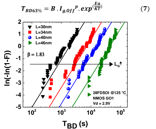
Figure 19. TDDB time to failure distribution for various L_G = 30 to 46nm from FDSOI N-FETs ( W_G = 1\mu m ) at fixed drain voltage V_{DS}=2.9V . Breakdown occurs later for longer devices.
